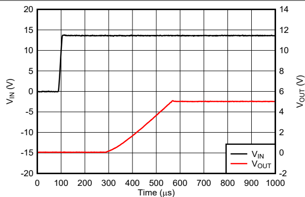
图 5-19. Start-Up Profile
