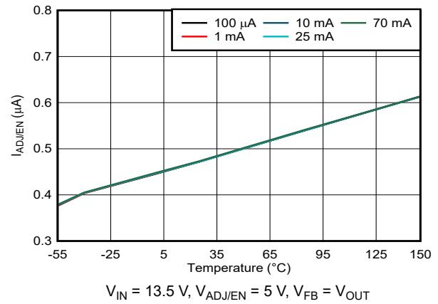
图 5-14. Adjustable Pin Current vs Ambient Temperature
