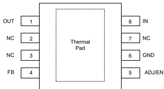
图 4-2. DDA Package, 8-Pin HSOIC (Top View)
