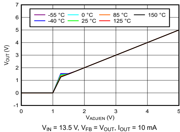
图 5-3. Output Voltage vs Adjustable Reference Voltage
