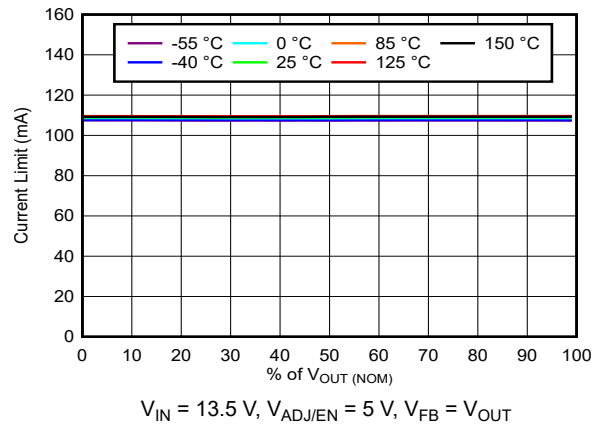
图 5-13. Current Limit vs Output Voltage
