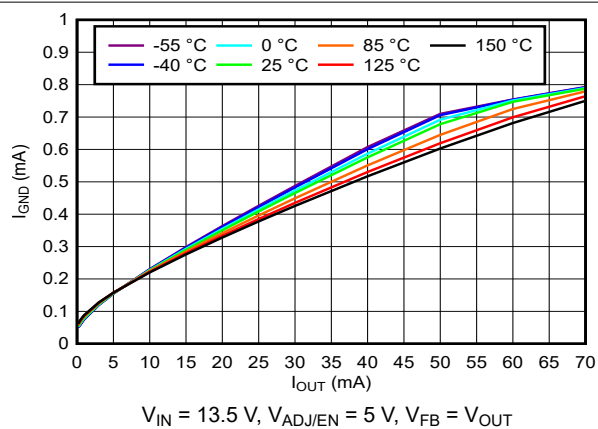
图 5-11. Ground Current vs Output Current
