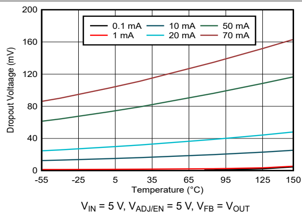
图 5-9. Dropout Voltage vs Ambient Temperature
