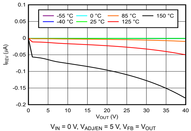
图 5-16. Reverse Current vs Output Voltage
