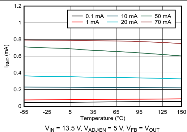
图 5-10. Ground Current vs Ambient Temperature
