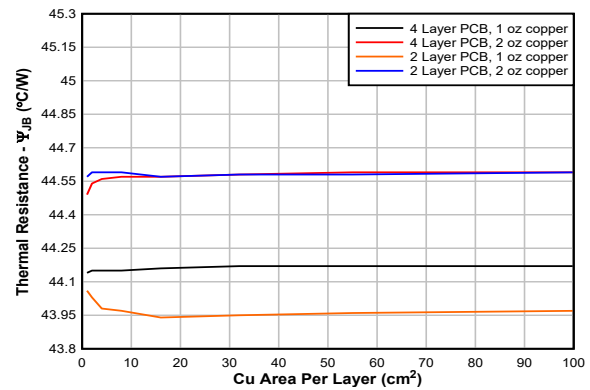
图 7-5. \psi_{JB} vs Copper Area (SOIC-8 Package)
