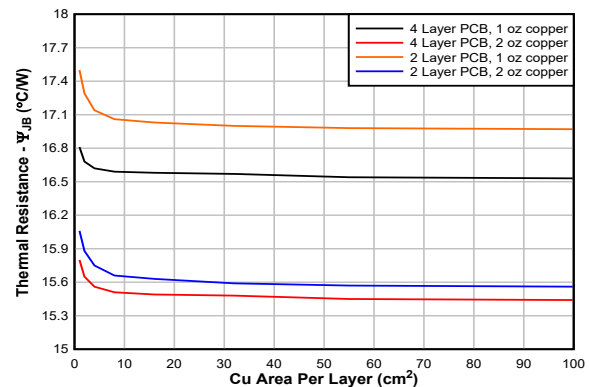
图 7-7. \psi_{JB} vs Copper Area (HSOIC-8 Package)
