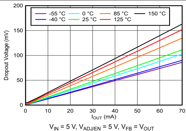
图 5-8. Dropout Voltage vs Load Current
