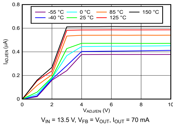
图 5-15. Adjustable Pin Current vs Adjustable Pin Voltage
