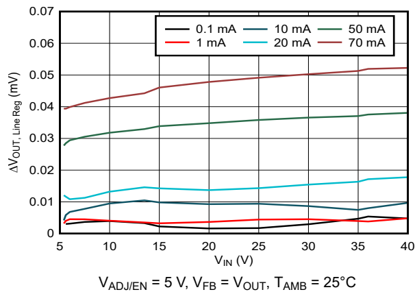
图 5-5. Line Regulation
