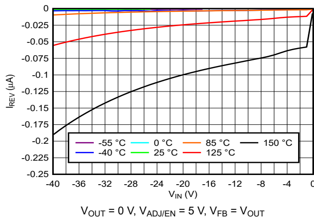
图 5-17. Reverse Current vs Input Voltage
