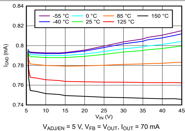
图 5-12. Ground Current vs Input Voltage
