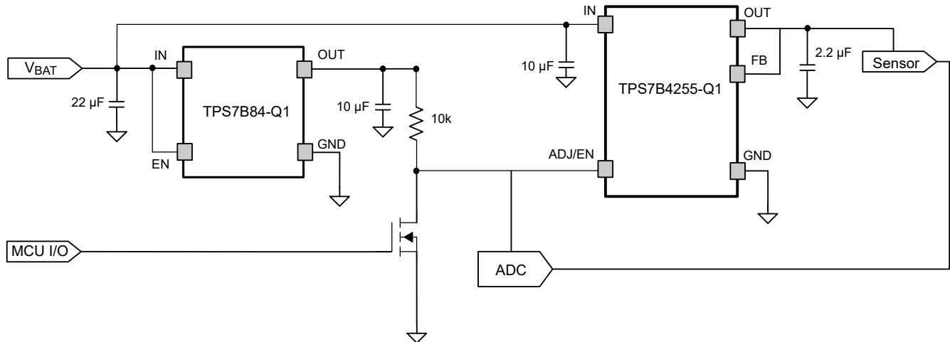
图 7-7. Tracking an LDO With an Enable Circuit
