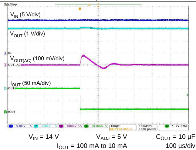
Figure 21. 100-mA to 10-mA Load Transient
