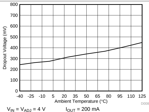
图 5. Dropout Voltage vs Ambient Temperature
