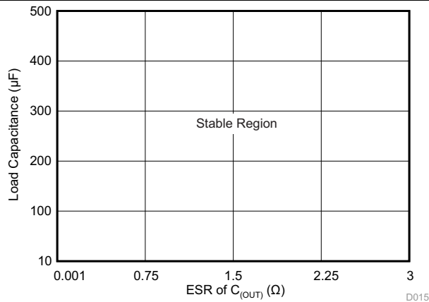
图 13. ESR Stability vs Load Capacitance
