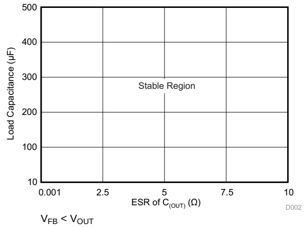
图 14. ESR Stability vs Load Capacitance
