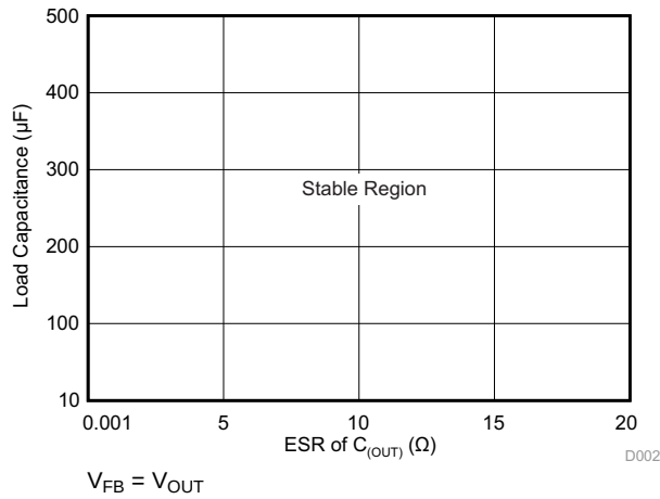
图 13. ESR Stability vs Load Capacitance
