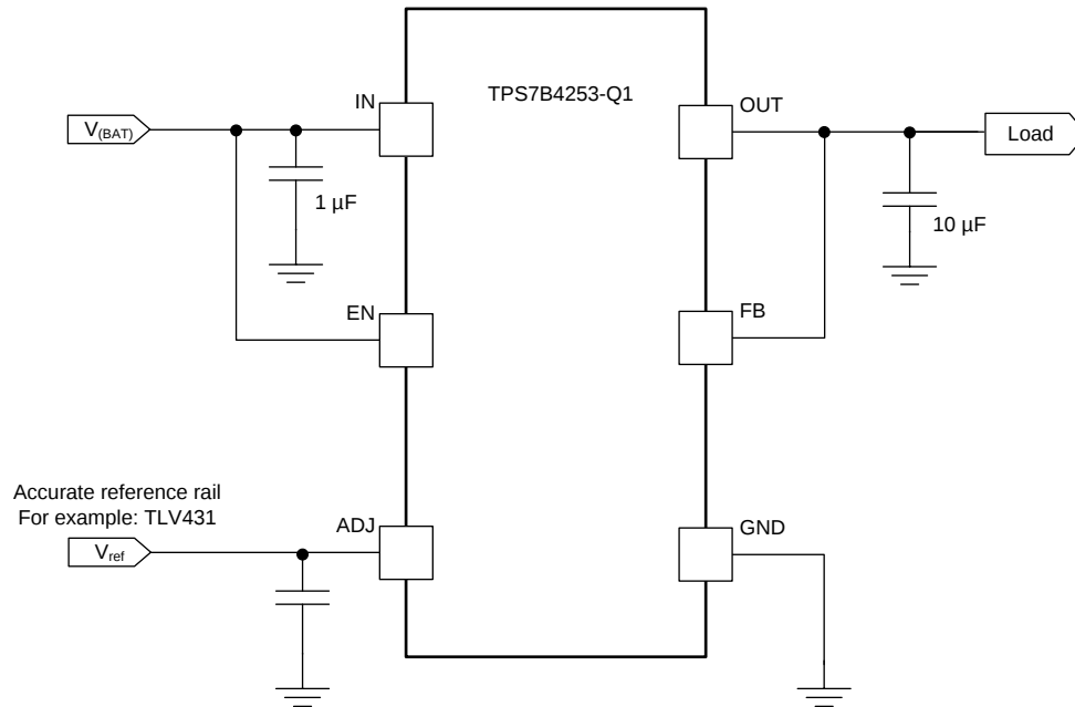
图 30. High-Accuracy LDO Application
