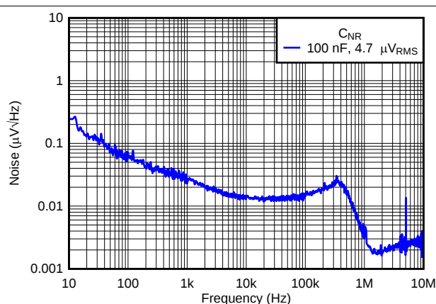
图 41. Output Noise vs Frequency
