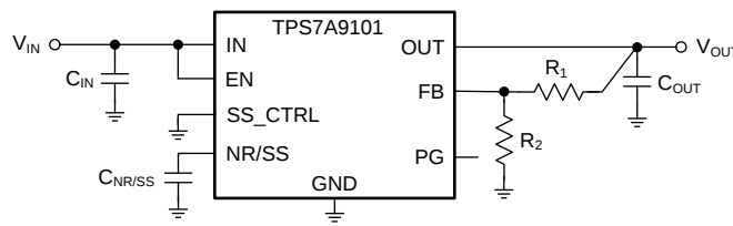
图 38. Adjustable Operation
