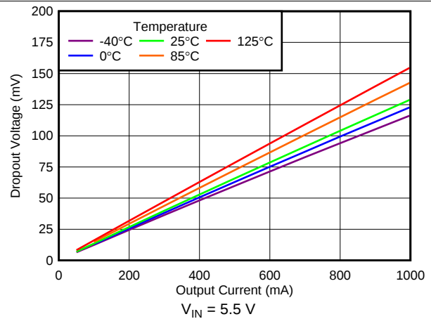
图 14. Dropout Voltage vs Output Current
