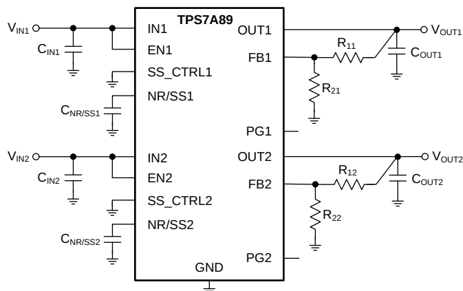
图 48. Adjustable Operation
