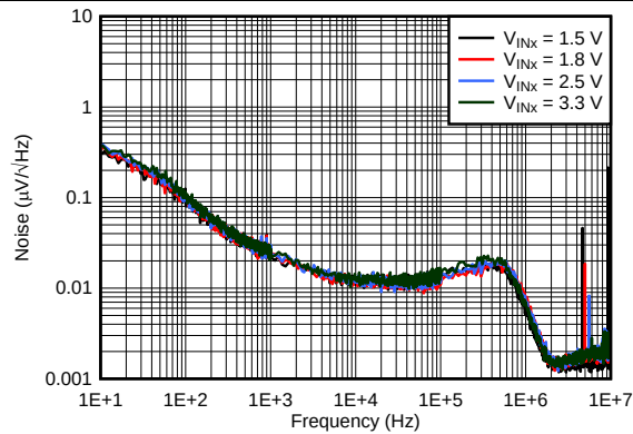
图 13. Noise vs Frequency and V_{\text{INX}}
