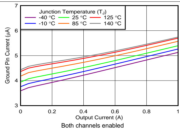
图 32. Ground Current vs Output Current
