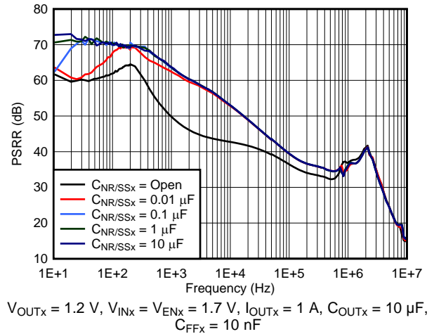
图 2. Power-Supply Rejection vs C_{NR/SSx}
