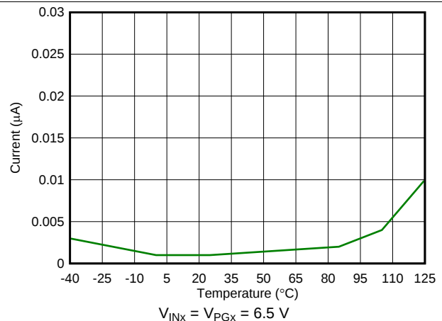
图 36. PG Leakage Current vs Temperature
