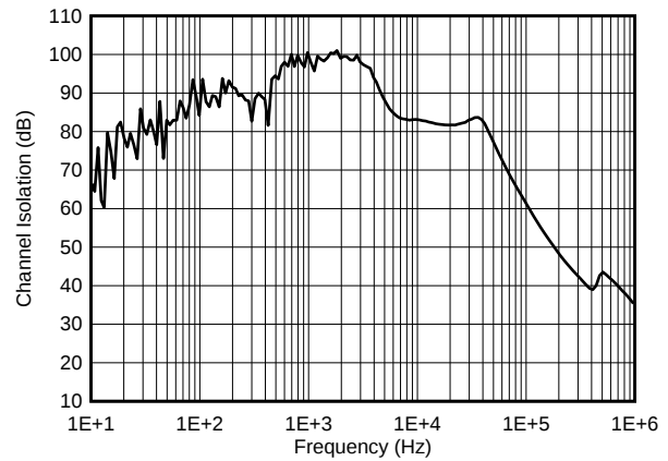
图 45. Channel-to-Channel Isolation
