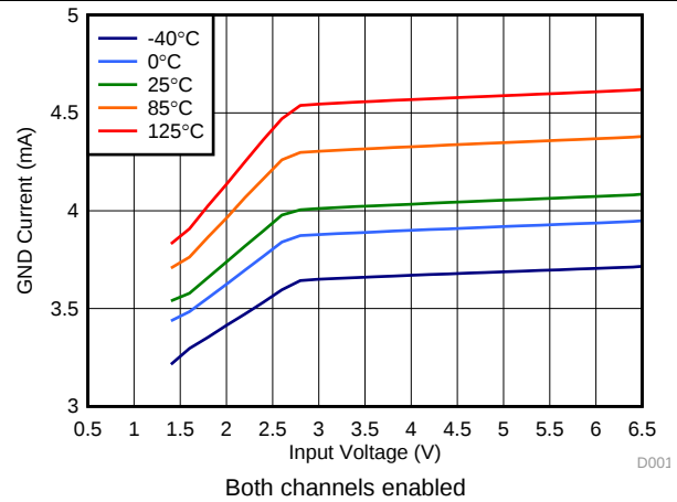
图 32. Ground Current vs Input Voltage
