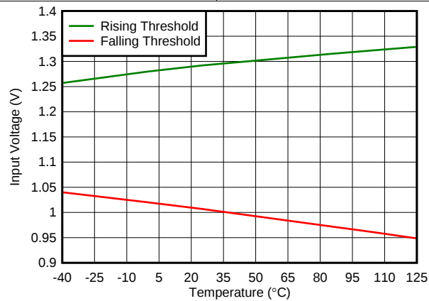
图 39. Enable Threshold vs Temperature ( V_{\text{INX}} = 1.4\text{ V} )
