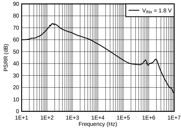
图 44. Power-Supply Rejection
