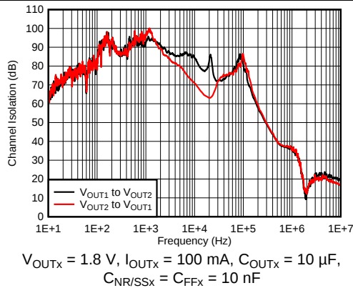
图 7. Channel-to-Channel Output Voltage Isolation vs Frequency
