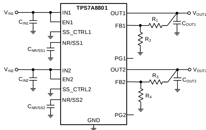
图 42. Adjustable Operation
