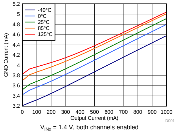
图 31. Ground Current vs Output Current
