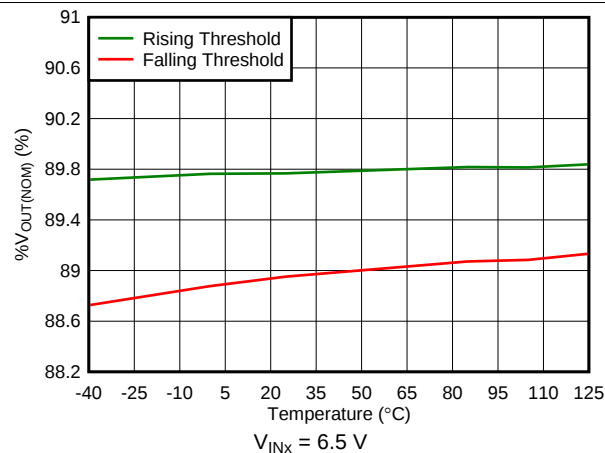
图 35. PG Threshold vs Temperature
