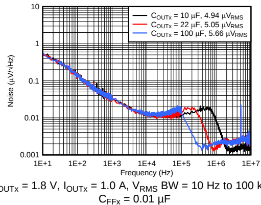
图 12. Spectral Noise Density vs C_{\text{OUTX}}
