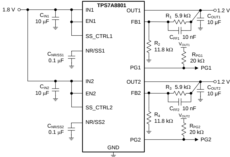
图 43. Application Example
