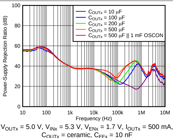
图 5. Power-Supply Rejection Ratio vs Frequency and Output Capacitance
