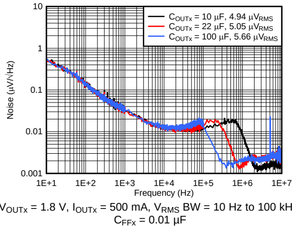
图 13. Noise vs Frequency and C_{\text{OUTX}}
