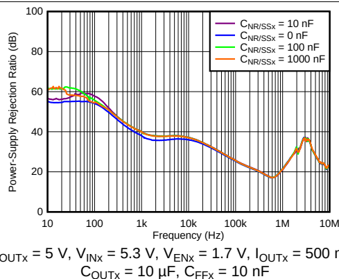
图 2. Power-Supply Rejection Ratio vs Frequency and C_{\text{NR/SSX}}
