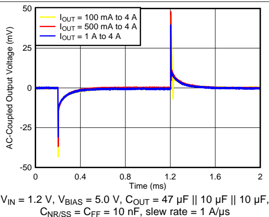
图 22. Load Transient Waveform vs Time and DC Load ( V_{OUT} = 0.9\text{ V} )
