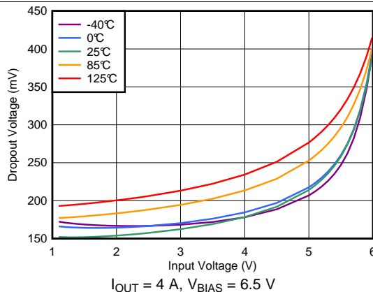
图 24. Dropout Voltage vs Input Voltage with Bias
