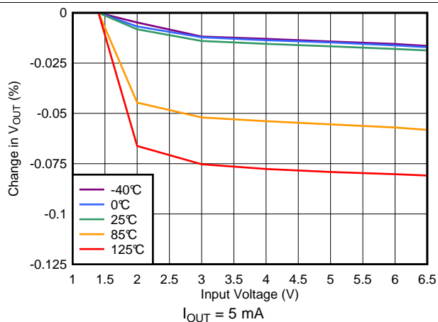
图 32. Line Regulation without Bias
