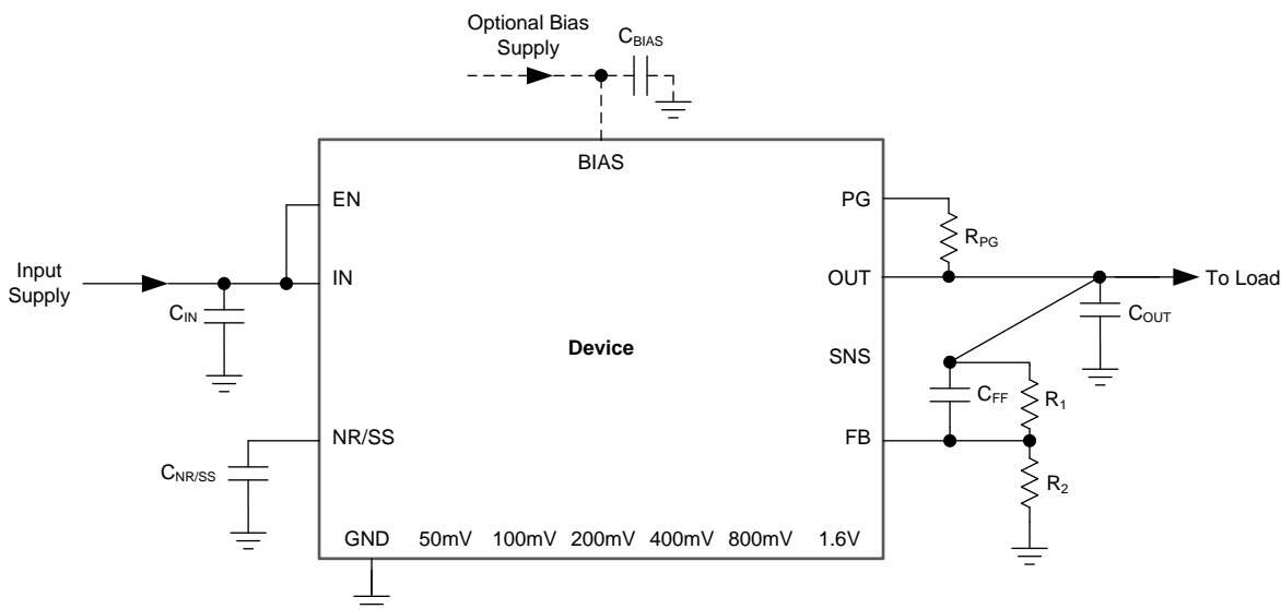
图 68. Typical Application
