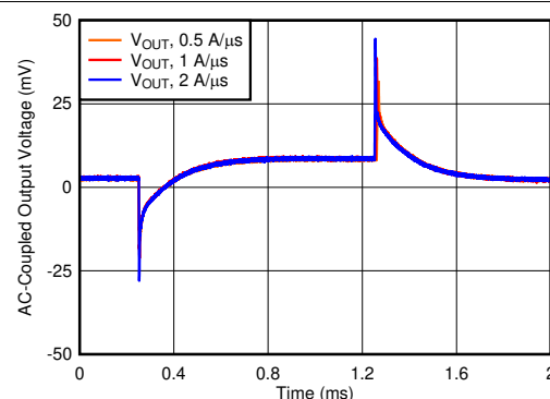
图 6-16. Load Transient vs Time and V_{OUT} With Bias
