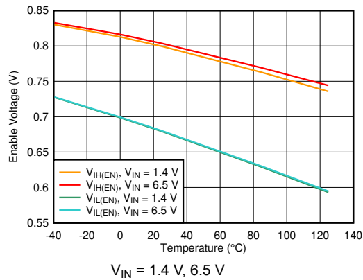
图 6-39. Enable Threshold vs Temperature
