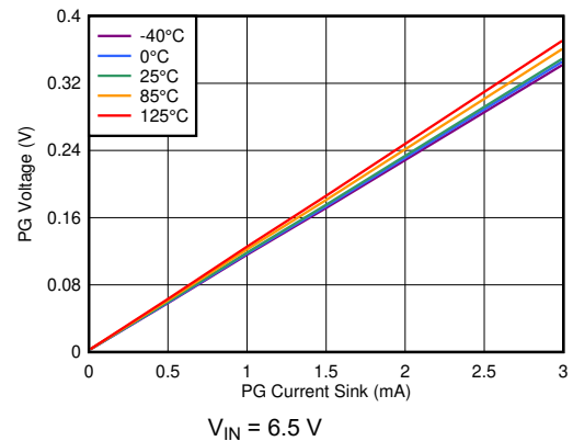
图 6-41. PG Voltage vs PG Current Sink
