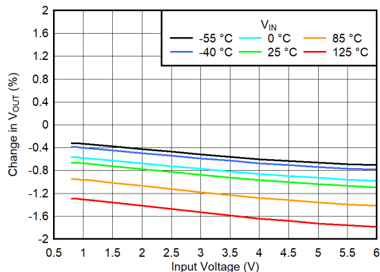
图 6-16. IN Line Regulation for V_{OUT} = 0.65\text{ V} , I_{OUT} = 0\text{ A}
