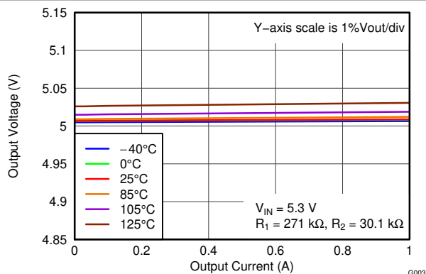
图 5-2. Load Regulation (5 V, Adjustable)
