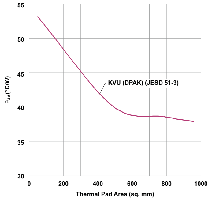
Figure 24. \theta_{JA} vs Thermal Pad Area
