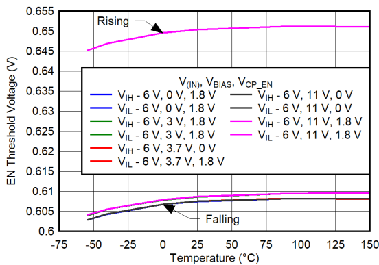
图 6-209. EN Threshold Voltage vs Temperature for V_{IN} = 6 V, V_{OUT} = 0.5 V
