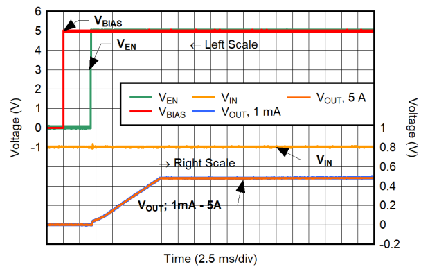
图 8-43. Start-Up Rail Sequence
