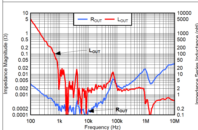
图 8-16. V_{IN} = 5.5 V, V_{OUT} = 5 V, V_{BIAS} = 8 V, CP_EN = 0, I_{OUT} = 5 A
