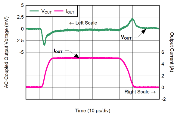
图 6-36. Load Transient for V_{OUT} = 5.2 V, I_{OUT} = 100 mA to 5 A, CP Enabled
