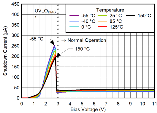
图 6-205. BIAS Pin Shutdown Current vs V_{BIAS} for V_{IN} = 6 V, V_{OUT(nom)} = 0.5 V, CP Disabled
