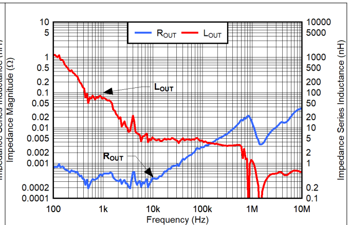
图 8-15. V_{IN} = 5.5 V, V_{OUT} = 5 V, V_{BIAS} = 8 V, CP_EN = 0, I_{OUT} = 500 mA
