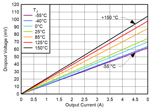
图 6-71. Dropout Voltage vs I_{OUT} for CP Disabled, V_{IN} = 0.7\text{ V} , V_{BIAS} = 3.9\text{ V}
