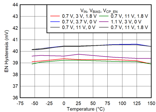
图 6-210. EN Hysteresis vs Temperature for V_{IN} = 0.7 V and 1.1 V, V_{OUT} = 0.5 V
