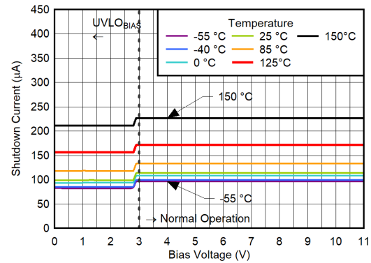
图 6-206. IN Pin Shutdown Current vs V_{BIAS} for V_{IN} = 6 V, V_{OUT(nom)} = 0.5 V, CP Disabled
