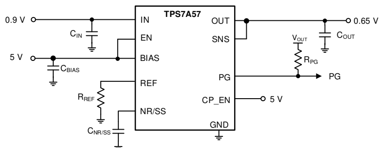
图 8-8. Typical Circuit
