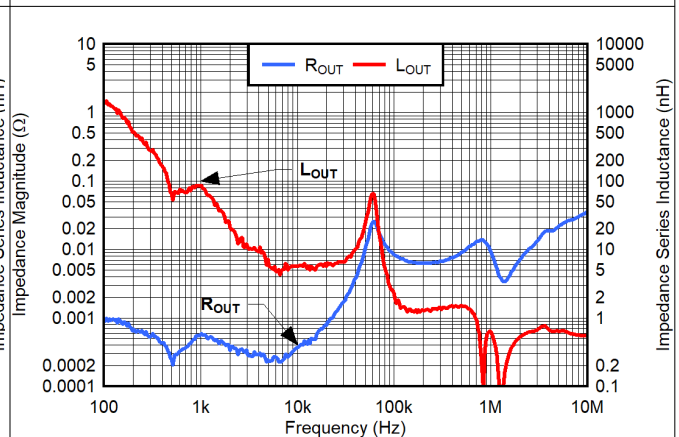
图 8-17. V_{IN} = 0.9 V, V_{BIAS} = 3 V, V_{OUT} = 0.5 V, CP_EN = 0, I_{OUT} = 4.6 A
