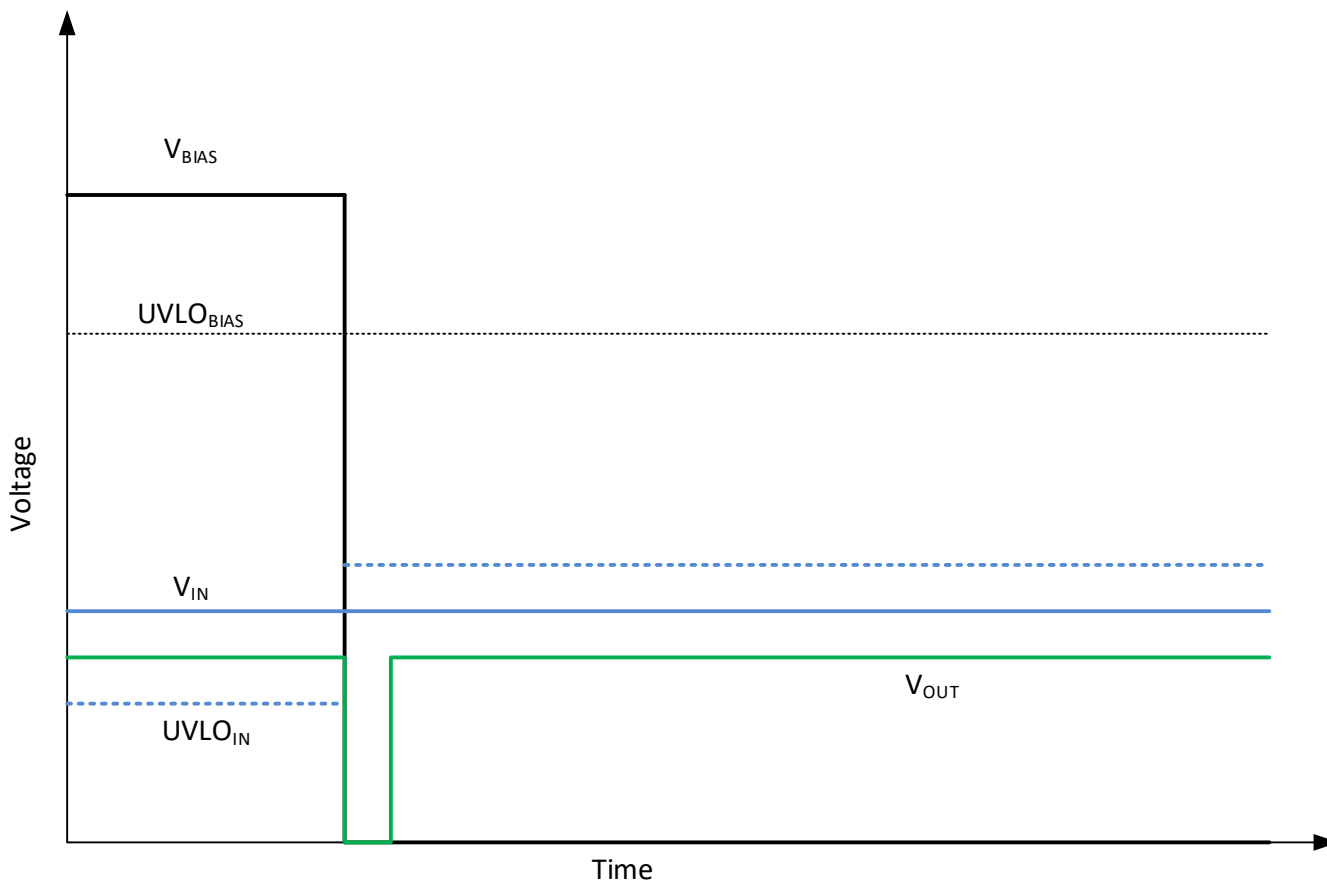
图 8-3. UVLO IN and UVLO BIAS Interaction
