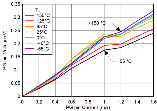
图 6-225. PG Pin Low-Level Voltage vs PG Pin Current for V_{IN} = 0.7\text{ V} , V_{BIAS} = 3\text{ V} , V_{CP\_EN} = 1.8\text{ V}
