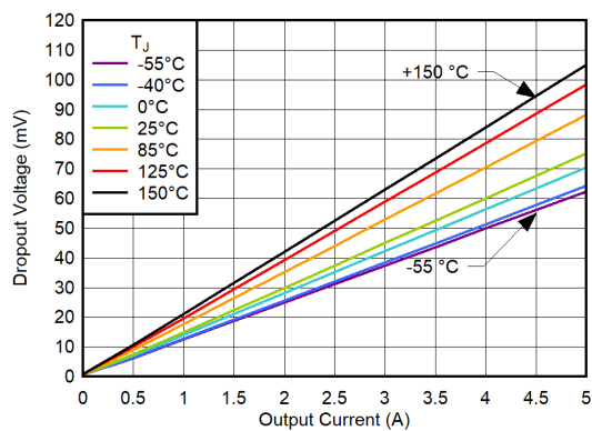
图 6-75. Dropout Voltage vs I_{OUT} for CP Enabled, V_{IN} = 6\text{ V} , No Bias
