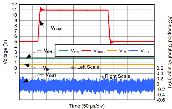
图 6-51. BIAS Line Transient for V_{IN} = 0.9\text{ V} to 6\text{ V} , I_{OUT} = 5\text{ A}
