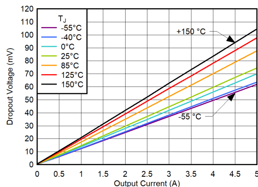
图 6-78. Dropout Voltage vs I_{OUT} for CP Disabled, V_{IN} = 5.3\text{ V} , V_{BIAS} = 9.2\text{ V}
