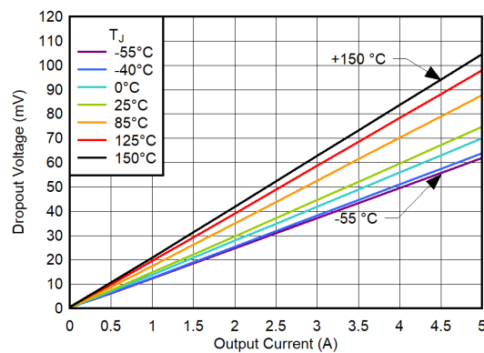
图 6-76. Dropout Voltage vs I_{OUT} for CP Enabled, V_{IN} = 5.3\text{ V} , V_{BIAS} = 3\text{ V}
