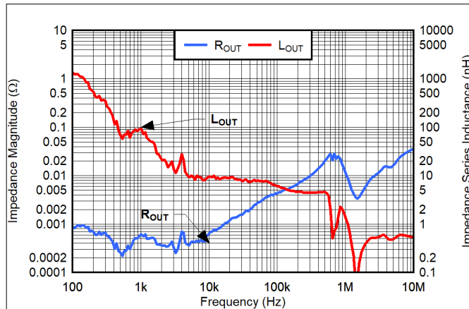
图 8-14. V_{IN} = 5.5 V, V_{OUT} = 5 V, V_{BIAS} = 8 V, CP_EN = 0, I_{OUT} = 200 mA
