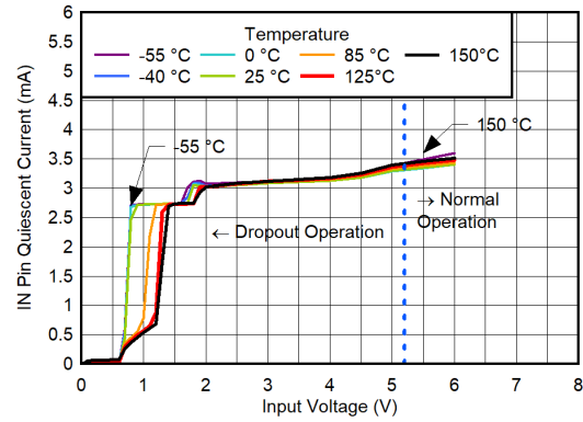
图 6-142. IN Pin Quiescent Current vs V_{IN} for V_{OUT} = 5.2\text{ V} , V_{BIAS} = 8.4\text{ V} , CP Disabled
