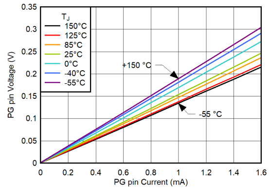
图 6-226. PG Pin Low-Level Voltage vs PG Pin Current for V_{IN} = 0.7\text{ V} , V_{BIAS} = 11\text{ V} , V_{CP\_EN} = 1.8\text{ V}
