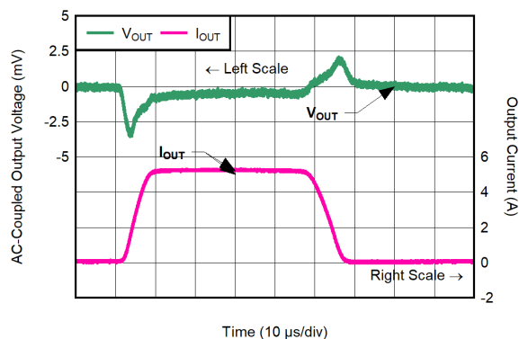
图 6-35. Load Transient for V_{OUT} = 3.3 V, I_{OUT} = 100 mA to 5 A, CP Enabled
