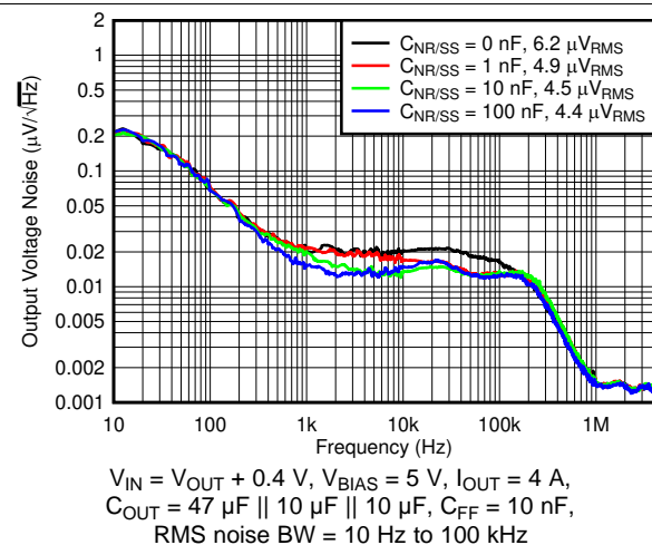
图 12. Output Noise vs Frequency and C_{NR/SS}
