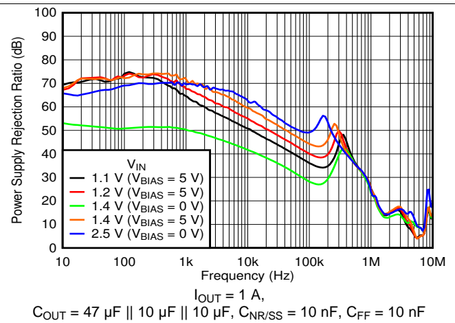
图 4. PSRR vs Frequency and V_{IN}
