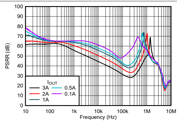
图 7-13. PSRR vs Frequency and I_{OUT}
