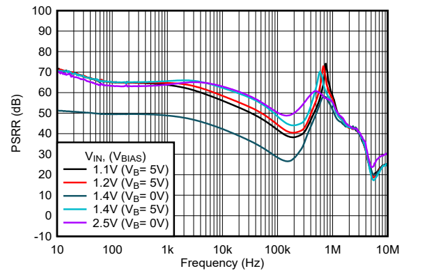
图 5-2. PSRR vs Frequency and V_{IN} With Bias
