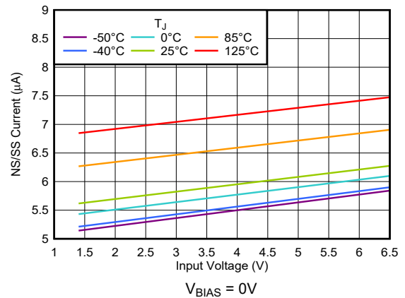
图 5-32. NR/SS Current vs Input Voltage
