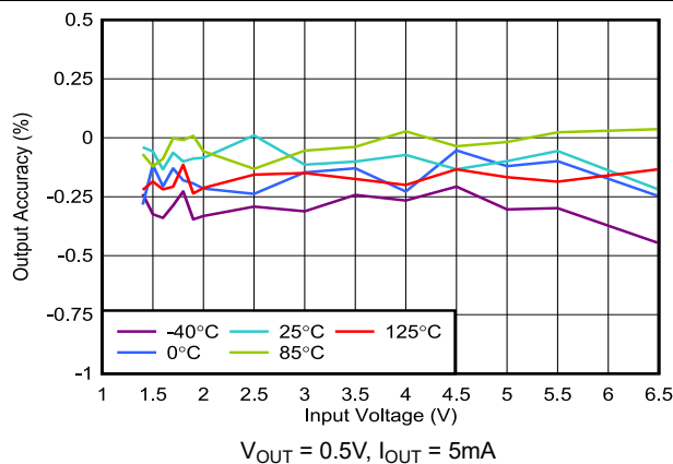
图 5-27. Line Regulation Without Bias
