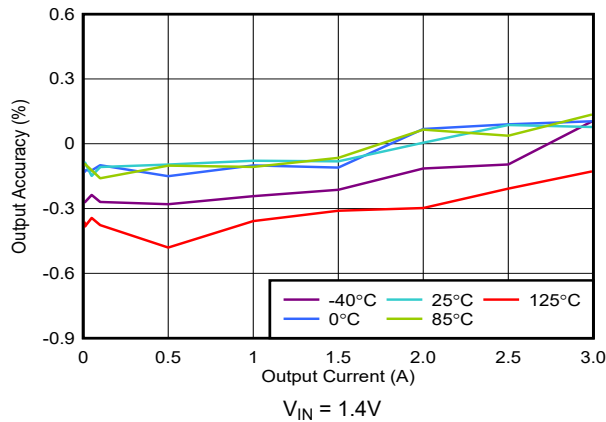
图 5-25. Load Regulation Without Bias
