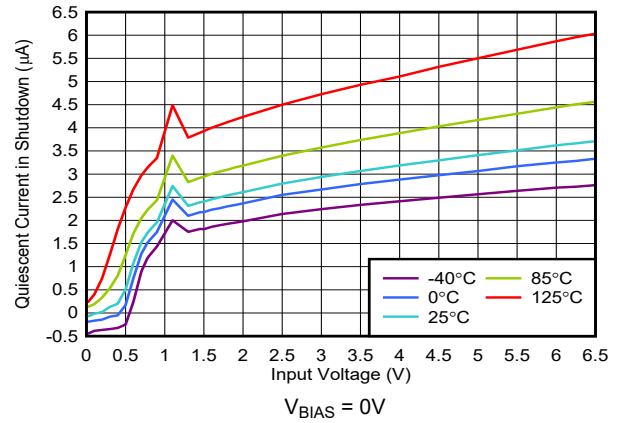
图 5-30. Shutdown Current vs Input Voltage
