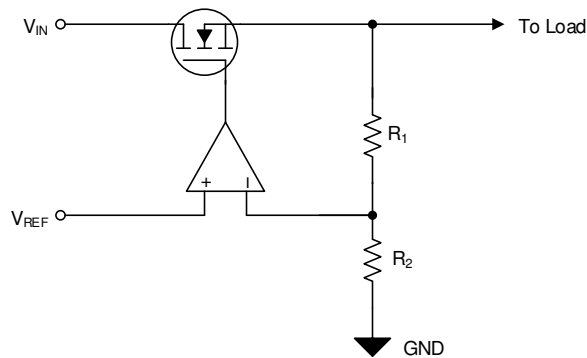
图 6-1. Simplified Regulation Circuit
