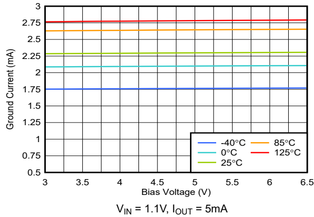
图 5-29. Quiescent Current vs Bias Voltage
