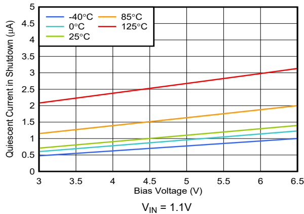
图 5-31. Shutdown Current vs Bias Voltage
