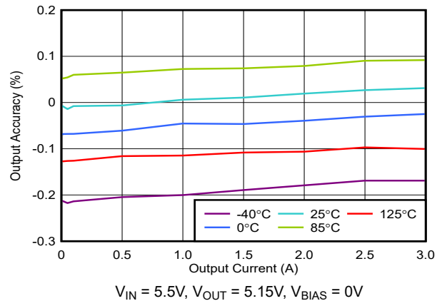
图 5-26. Load Regulation Without Bias
