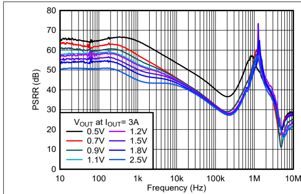
图 7-12. PSRR vs Frequency and V_{OUT} With Bias
