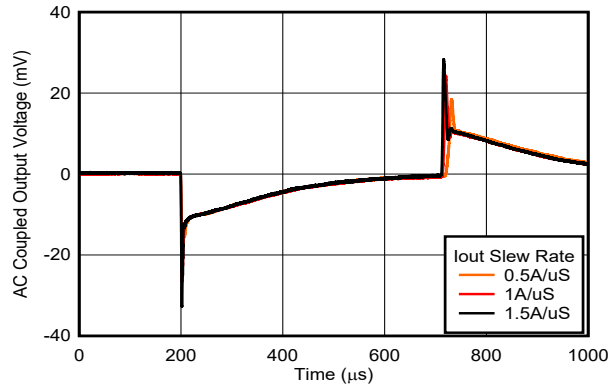
图 5-17. Load Transient vs Time and Slew Rate
