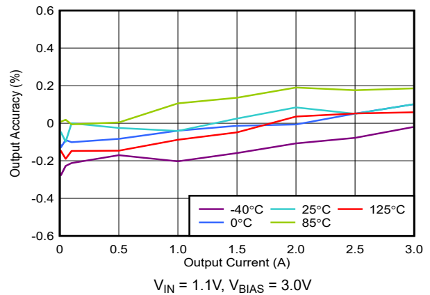
图 5-24. Load Regulation With Bias
