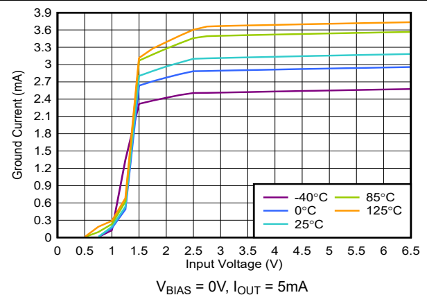
图 5-28. Quiescent Current vs Input Voltage
