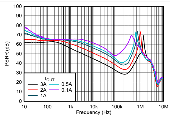
图 7-13. PSRR vs Frequency and I_{OUT}
