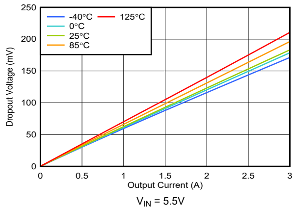
图 5-23. Dropout Voltage vs Output Current (High V_{IN} )
