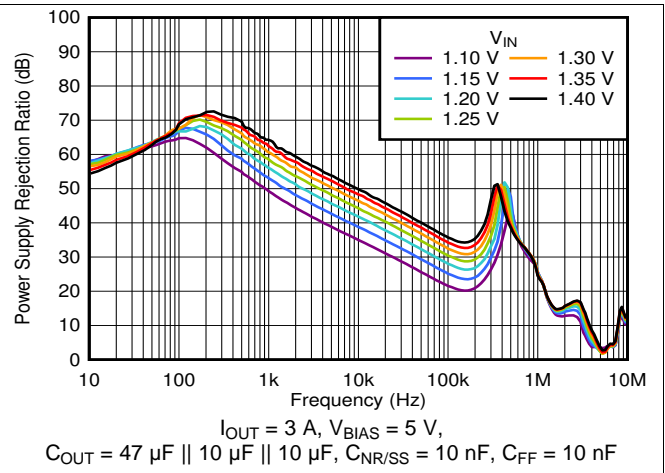
图 2. PSRR vs Frequency and V_{IN} With Bias
