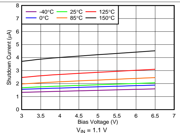
图 30. Shutdown Current vs Bias Voltage
