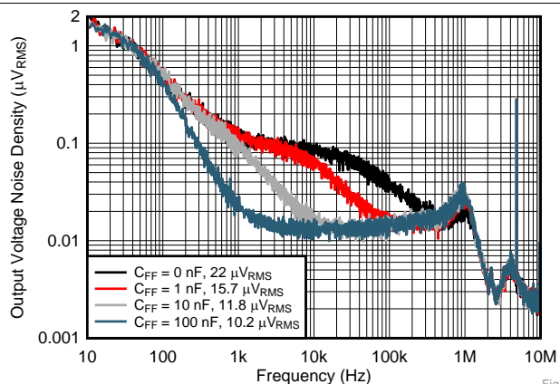
V_{IN} = V_{OUT} + 0.3\text{ V} , V_{BIAS} = 5\text{ V} , I_{OUT} = 2\text{ A} , sequencing with a dc-dc converter and PG, C_{NR/SS} = 10\text{ nF} , RMS noise BW = 10 Hz to 100 kHz
