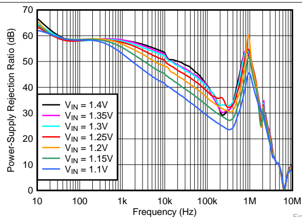
图 2. PSRR vs Frequency and V_{IN} With Bias
