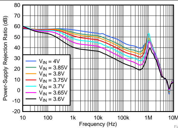
图 4. PSRR vs Frequency and V_{IN}
