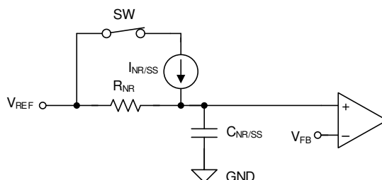
图 2. Simplified Soft-Start Circuit
