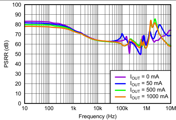
Figure 13. Power-Supply Rejection Ratio vs Frequency and I_O
