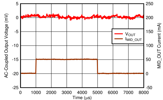
图 6-32. Load Transient (MID_OUT)
