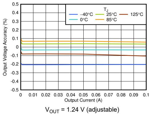
图 6-1. V_{\text{OUT}} Accuracy vs I_{\text{OUT}}
