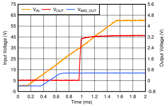
图 6-13. Slow Start-Up
