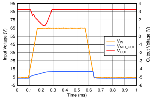
图 6-25. Line Transient ( V_{\text{MID\_OUT}} in Dropout)
