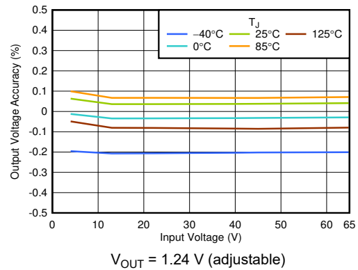
图 6-2. V_{\text{OUT}} Accuracy vs V_{\text{IN}}
