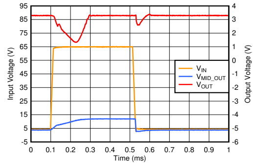
图 6-26. Line Transient ( V_{\text{MID\_OUT}} in Dropout)
