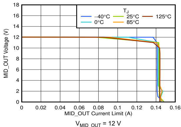
图 6-5. V_{\text{MID\_OUT}} vs I_{\text{CL}}(\text{MID\_OUT})
