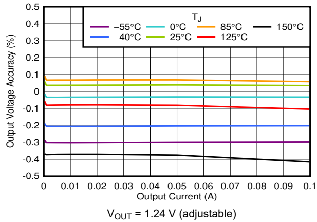
图 6-1. V_{\text{OUT}} Accuracy vs I_{\text{OUT}}
