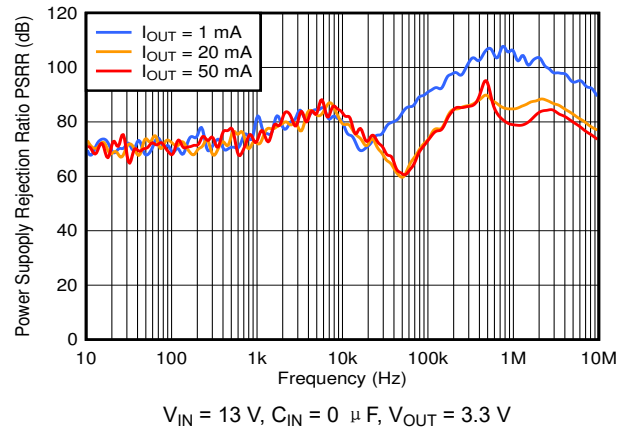
图 6-32. OUT PSRR vs Frequency and I_{OUT}
