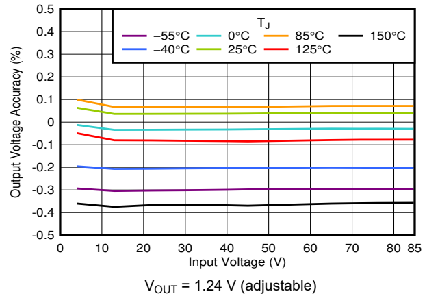
图 6-2. V_{\text{OUT}} Accuracy vs V_{\text{IN}}
