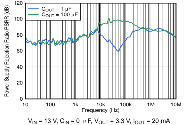
图 6-34. OUT PSRR vs Frequency and C_{OUT}
