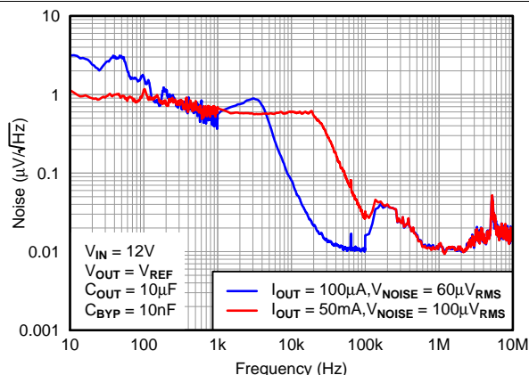
Figure 9. Output Spectral Noise Density
