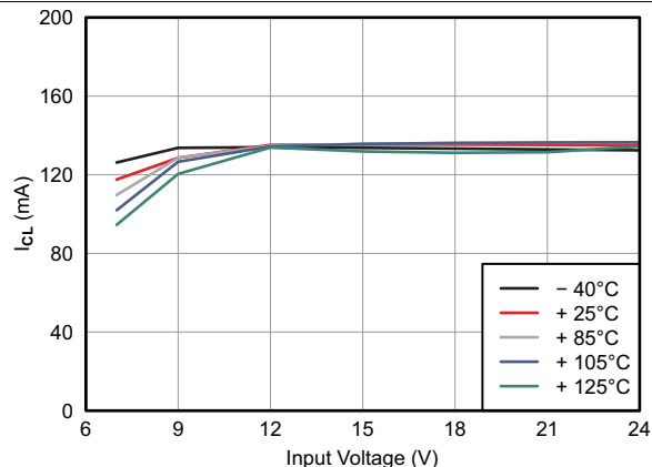
Figure 10. Current Limit
