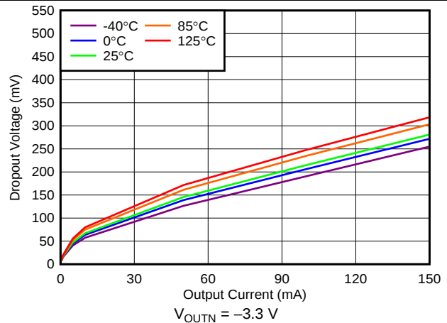
图 51. Negative Regulator Dropout Voltage vs Output Current
