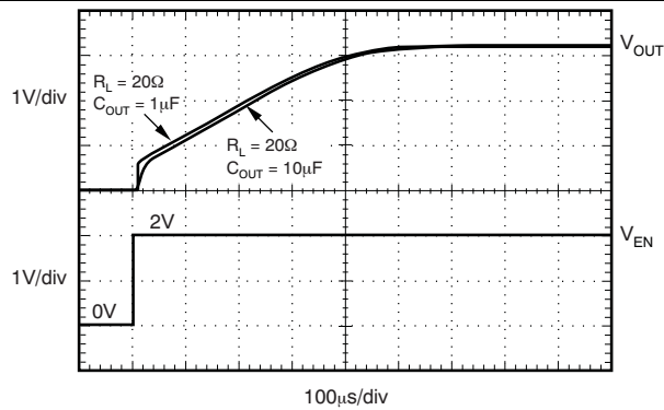
Figure 32. TPS7A3701: Turn-on Response
