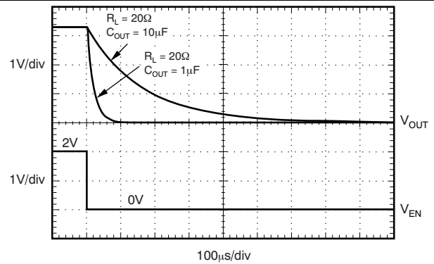
Figure 33. TPS7A3701: Turn-off Response
