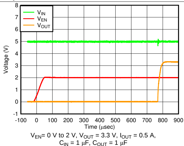
图 32. Start-Up With Enable
