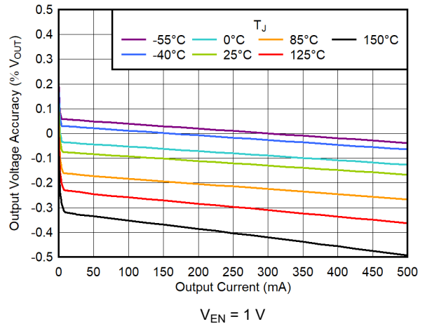
图 6-2. Output Voltage Accuracy vs I_{OUT}
