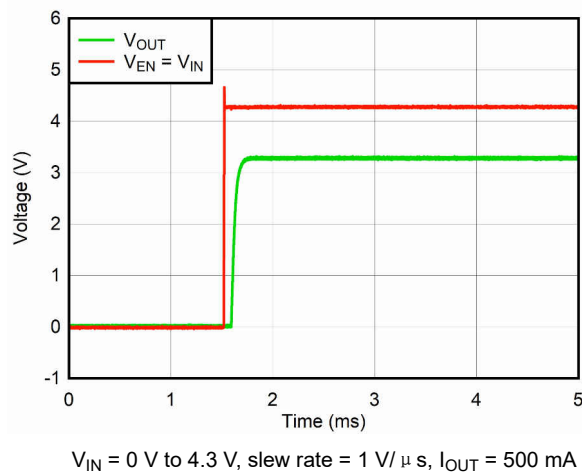
图 6-23. Start-Up With V_{EN} = V_{IN}
