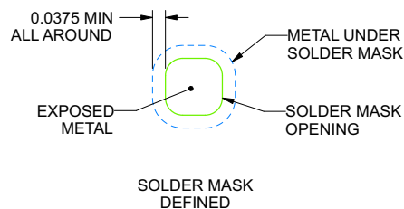
SOLDER MASK DETAILS NOT TO SCALE
