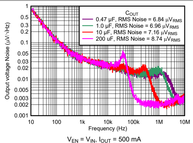
图 6-42. Noise vs Frequency and C_{OUT}
