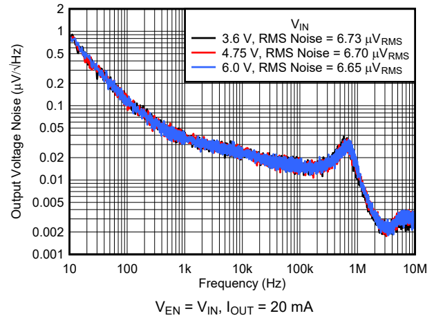
图 6-38. Noise vs Frequency and V_{IN}
