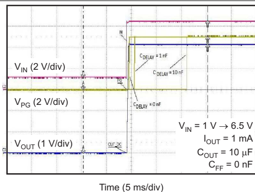
Figure 13. Power-Good Delay
