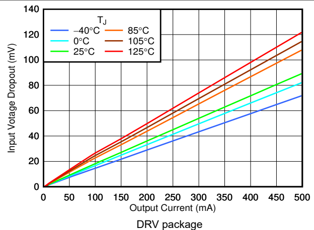
图 6-4. V_{IN} Dropout vs I_{OUT} and Temperature
