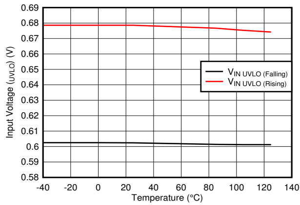
图 6-31. V_{UVLO(IN)} Rising and Falling Threshold vs Temperature
