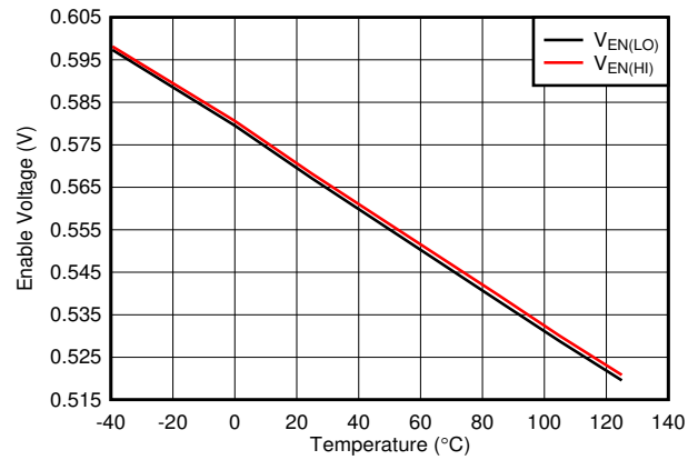
图 6-32. Enable High and Low Threshold vs Temperature
