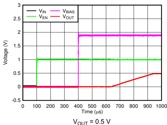
图 6-17. Startup With V_{BIAS} Powering Up After V_{IN} and V_{EN}
