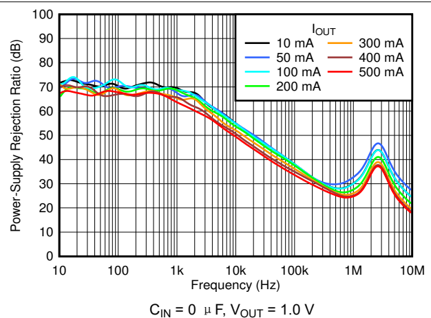
图 6-24. V_{IN} PSRR vs Frequency and I_{OUT}
