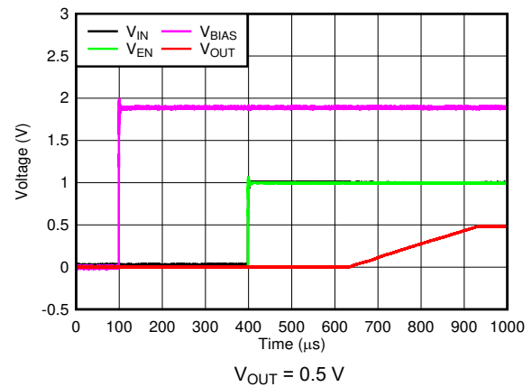
图 6-14. Startup With V_{EN} = V_{IN}
