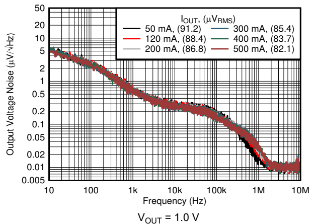
图 6-28. Output Noise vs Frequency and I_{OUT}
