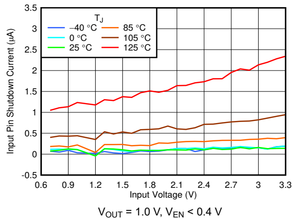
图 6-13. I_{SHDN} vs V_{IN} and Temperature
