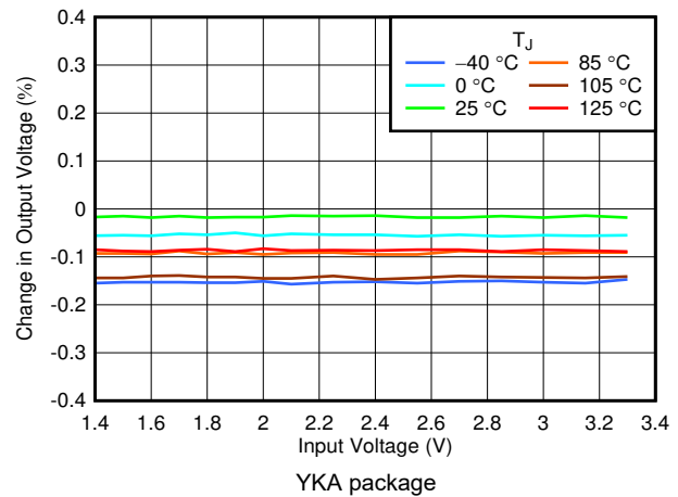
图 6-2. Output Accuracy vs V_{IN} and Temperature
