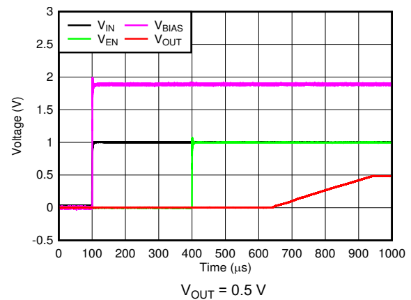
图 6-16. Startup With Separated V_{EN}
