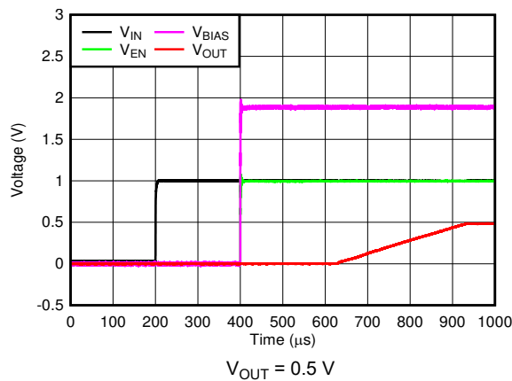
图 6-15. Startup With V_{EN} and V_{BIAS} Powering Up Simultaneously
