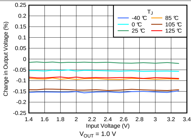
图 1. Output Accuracy Over Temperature, YKA Package
