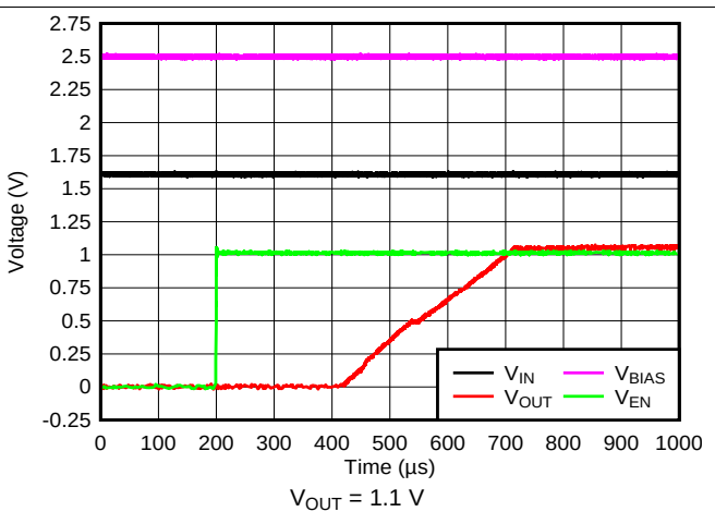
图 22. Startup With Separated V_{EN}
