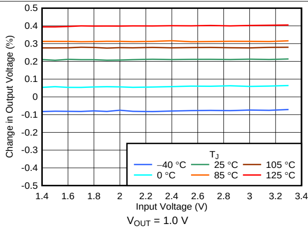
图 3. Output Accuracy Over Temperature, DSE Package
