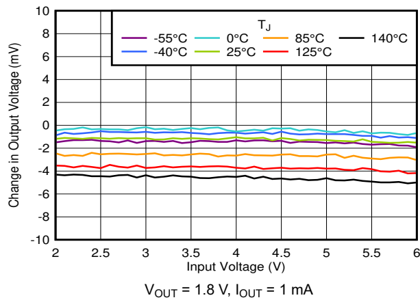
图 6-25. Line Regulation vs V_{IN} and Temperature
