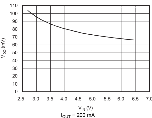
Figure 7. Dropout vs Input Voltage
