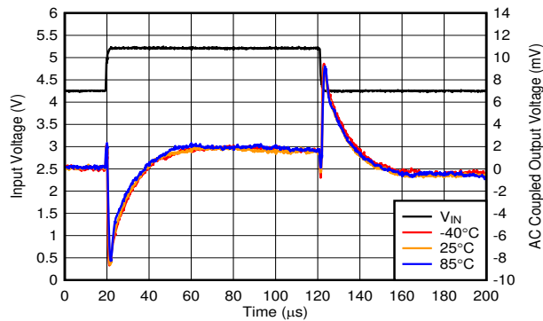
图 6-19. Line Transient vs Temperature
