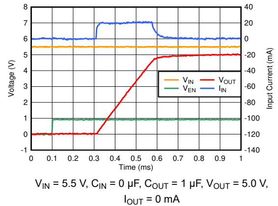
图 6-28. Start-Up Inrush Current With C_{OUT} = 1\text{ }\mu\text{F}
