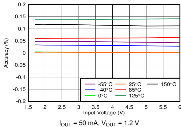
图 6-3. Output Accuracy vs V_{\text{IN}}
