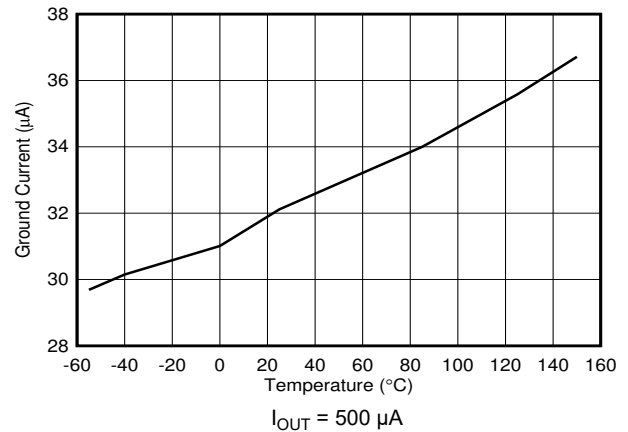
图 6-10. 500- \mu\text{A} Ground Current vs Temperature
