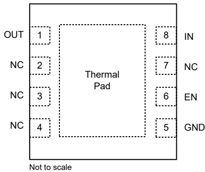
图 5-3. DRB Package (Fixed) B Version, 8-Pin VSON (Top View)
