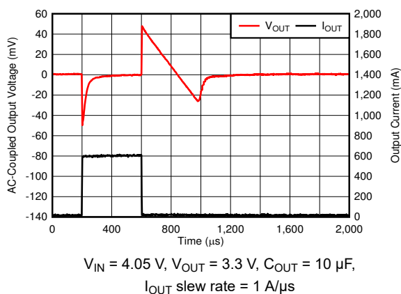
图 8-9. I_{\text{OUT}} Transient From 1 mA to 600 mA
