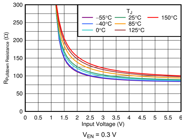
图 6-13. Pulldown Resistor ( R_{\text{Pulldown}} ) vs V_{\text{IN}}
