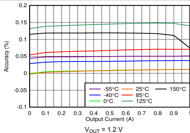
图 6-5. Output Accuracy vs Output Current
