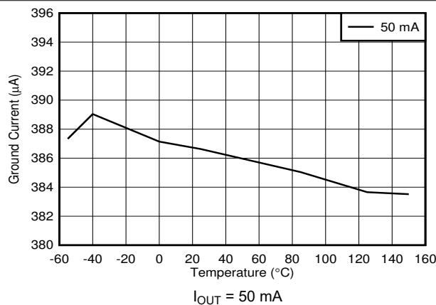
图 6-11. 50-mA Ground Current vs Temperature
