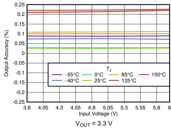
图 6-1. Output Accuracy vs V_{\text{IN}}
