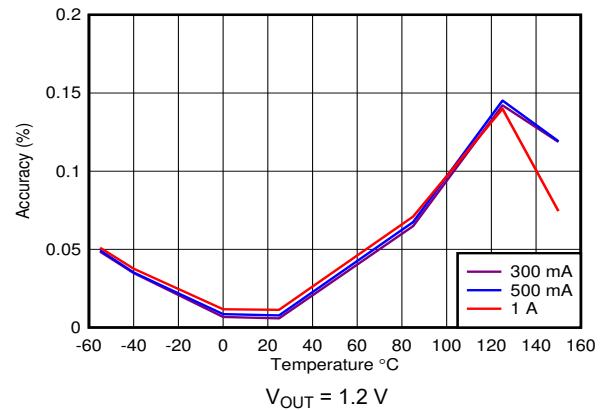
图 6-4. Output Accuracy vs Temperature
