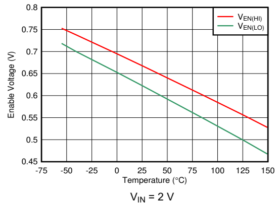
图 6-14. V_{\text{EN(HI)}} and V_{\text{EN(LO)}} Thresholds vs Temperature
