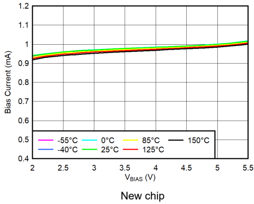
图 5-25. BIAS Pin Current vs V_{BIAS} and Temperature ( T_J )
