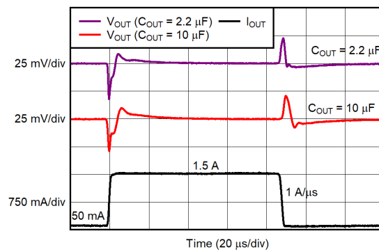
New chip 图 5-37. Output Load Transient Response
