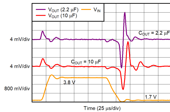
New chip 图 5-35. V_{IN} Line Transient
