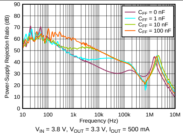
图 38. PSRR vs Frequency and C_{FF}
