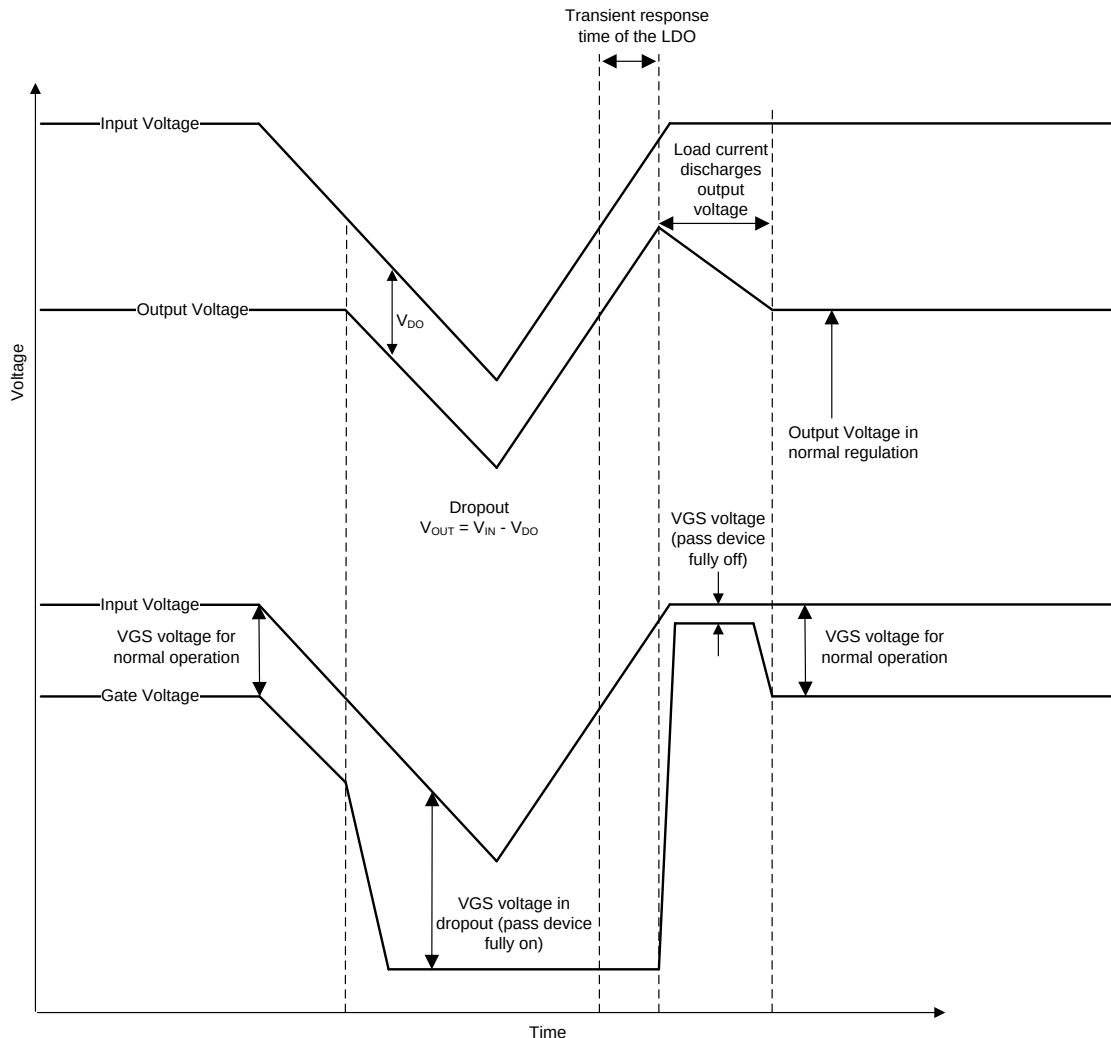
图 48. Line Transients From Dropout
