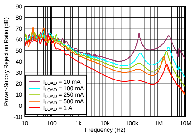
图 51. PSRR vs Frequency and I_{LOAD}
