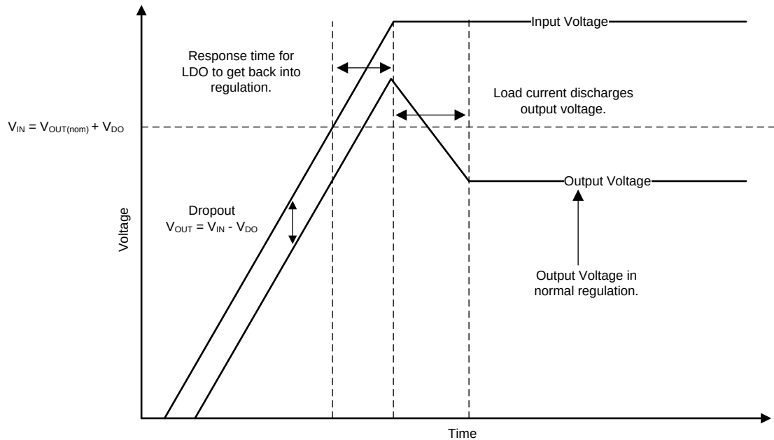
图 47. Startup Into Dropout
