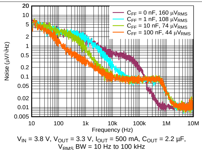
图 42. Output Spectral Noise Density vs Frequency and C_{FF}
