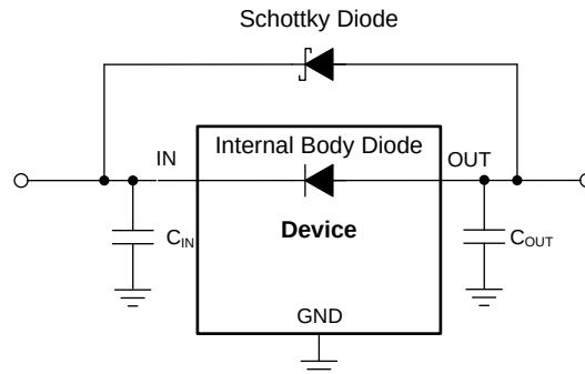
图 49. Example Circuit for Reverse Current Protection Using a Schottky Diode
