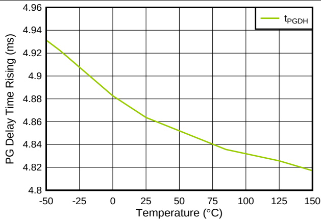
图 19. t_{PGDH} vs Temperature (For TPS746B Only)
