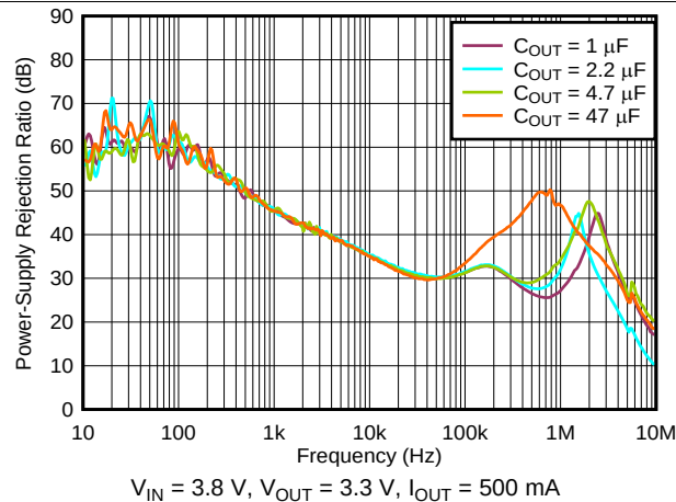
图 37. PSRR vs Frequency and C_{OUT}
