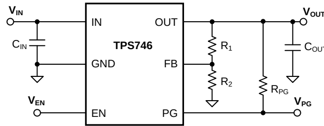
图 50. TPS746 Typical Application
