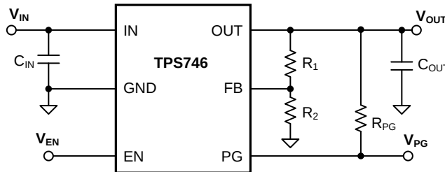
图 46. Adjustable Operation
