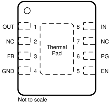
图 5-3. DRB Package, 8-Pin Adjustable VSON (Top View)
