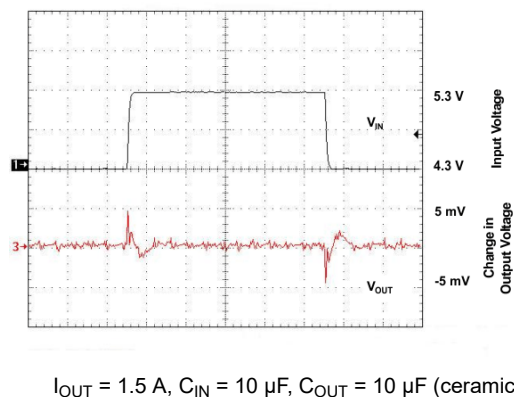
图 5-23. Line Transient Response
