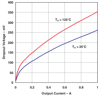
图 5-1. Dropout Voltage vs Output Current
