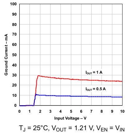
图 5-6. Ground Current vs Input Voltage
