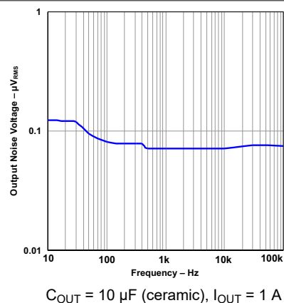
图 5-20. Output Noise Voltage vs Frequency
