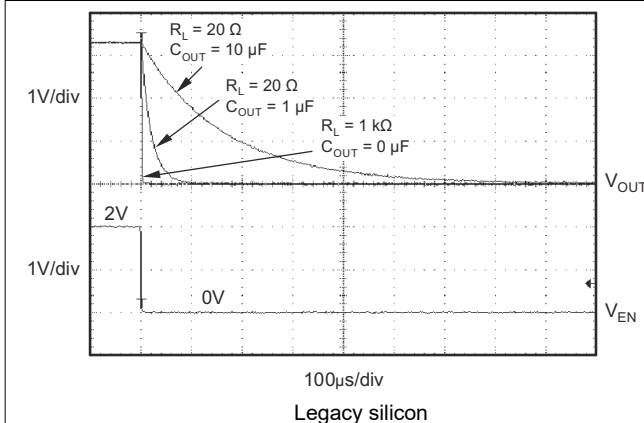
图 5-41. TPS73633 Turn-Off Response
