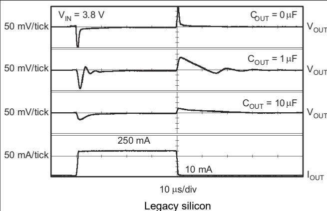
图 5-35. TPS73233 Load Transient Response
