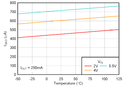
图 5-14. Ground Pin Current vs Temperature
