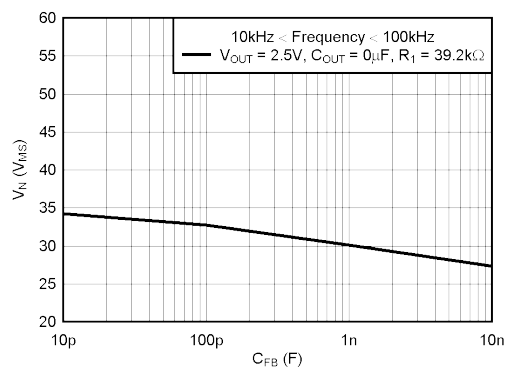
图 7-8. TPS73201 RMS Noise Voltage vs C_{FB}
