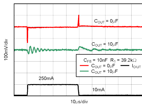
图 5-52. TPS73201 Load Transient, Adjustable Version
