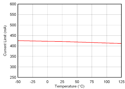
图 5-22. Current Limit vs Temperature
