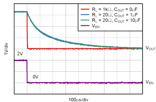
图 5-42. TPS73233 Turn-Off Response
