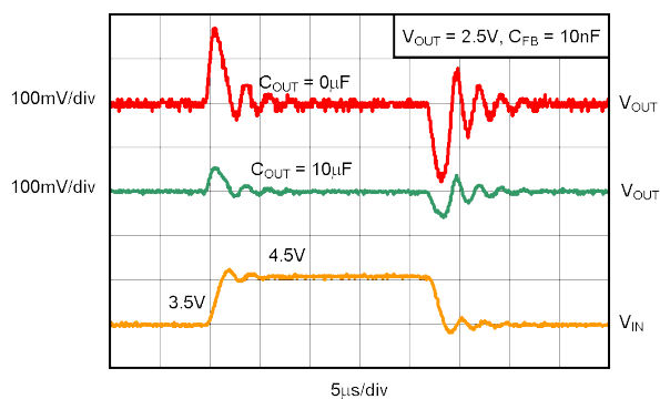
图 5-54. TPS73201 Line Transient, Adjustable Version
