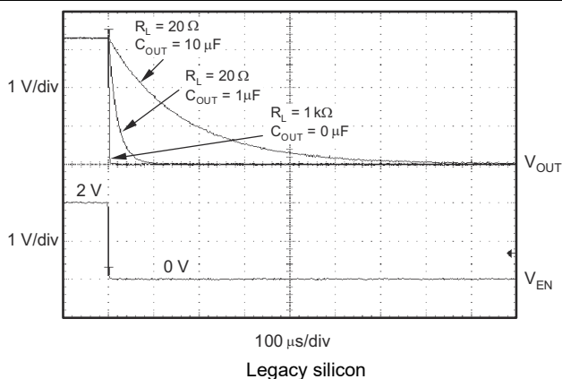
图 5-41. TPS73233 Turn-Off Response
