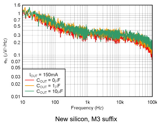
图 5-28. Noise Spectral Density C_{NR} = 0\ \mu\text{F}
