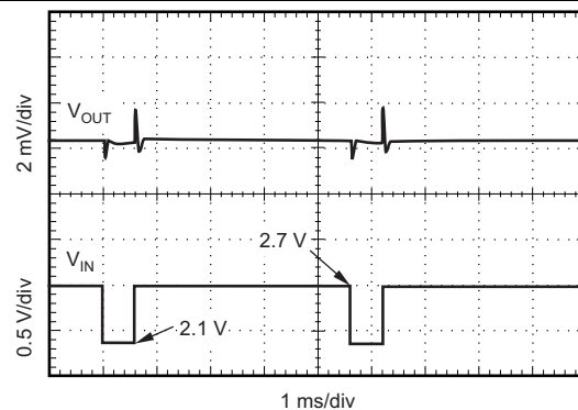
Figure 31. Line Transient Response (TPS72718)
