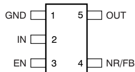
DBV Package 5-Pin SOT23 Top View
