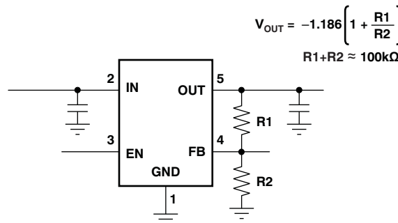
Figure 27. TPS72301 Adjustable LDO Regulator Programming
