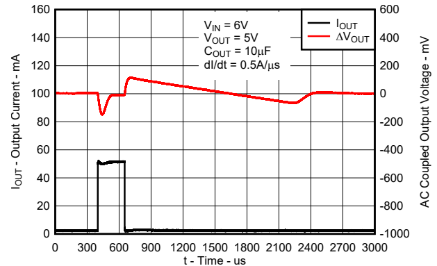
图 8-9. Load Transient Response for New Chip
