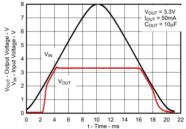
图 8-5. Power-Up and Power-Down for New Chip
