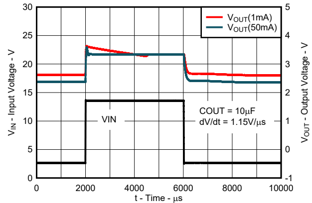
图 8-11. Fast Line Transient Response for New Chip
