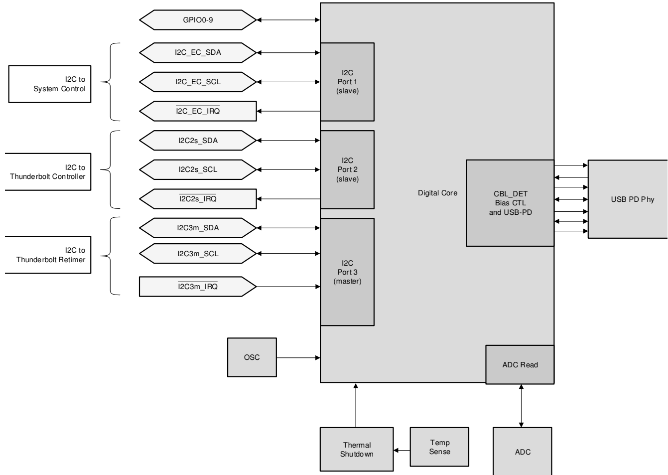
图 8-21. Digital Core Block Diagram
