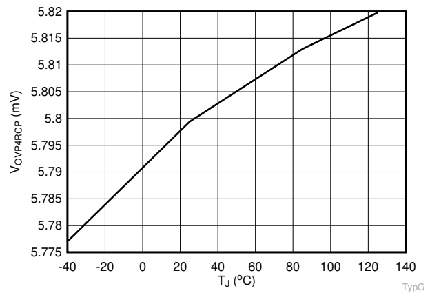
图 6-4. V OVP4RCP (Setting 2) vs. Temperature
