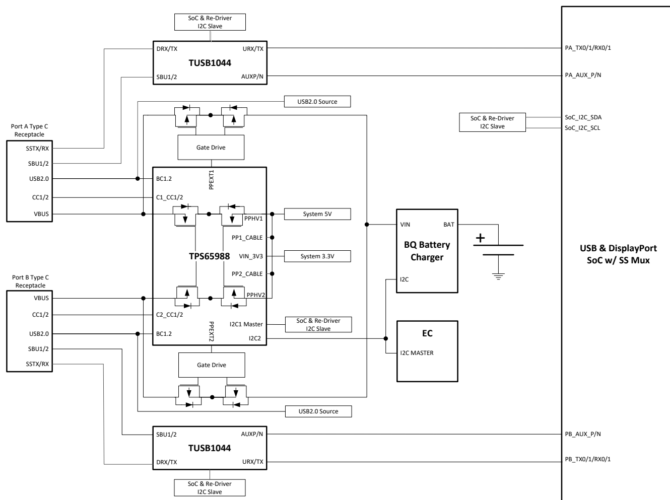
图 9-10. TPS65988 and SoC & Redriver I2C
