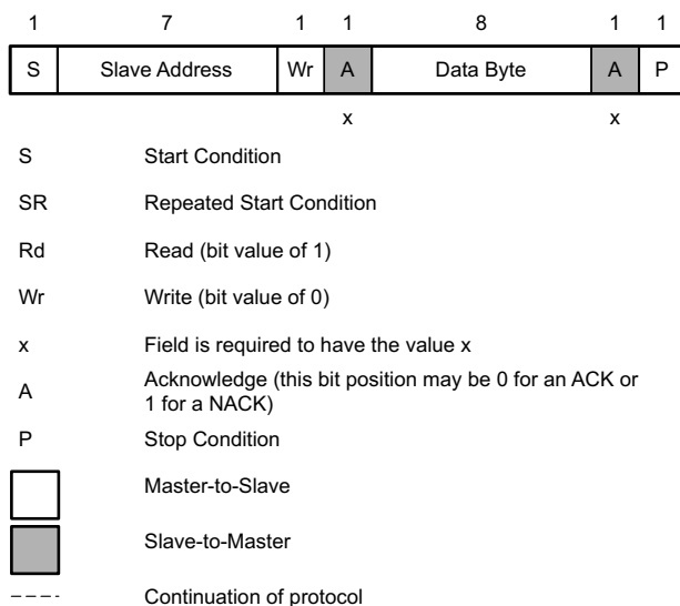
图 9-67. I 2 C Read/Write Protocol Key
