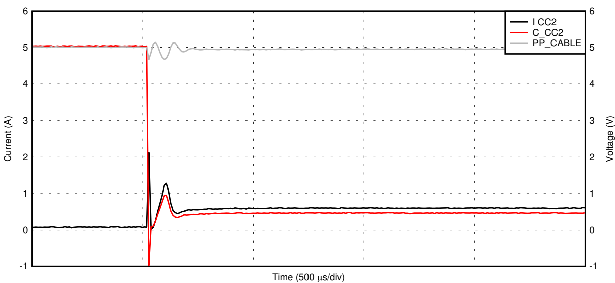
图 9-32. PP_CABLE to C_CCn Current Limit With a Hard Short (Extended Time Base)
