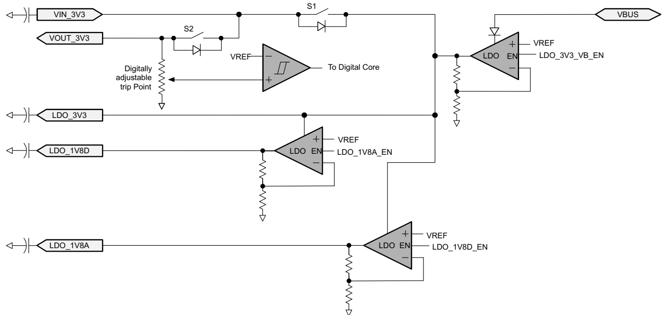
图 9-40. Power Supply Path
