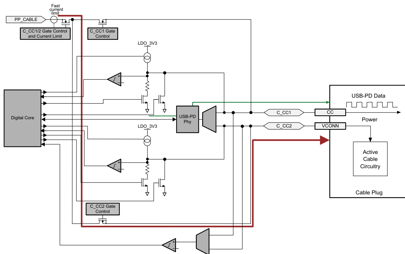
图 9-29. Port C_CC1 and C_CC2 Normal Orientation Power from PP_CABLE
