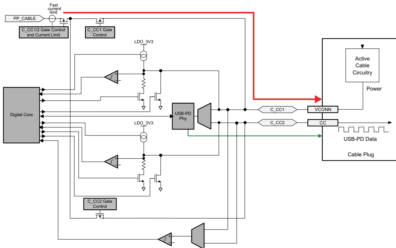
图 9-30. Port C_CC1 and C_CC2 Reverse Orientation Power from PP_CABLE
