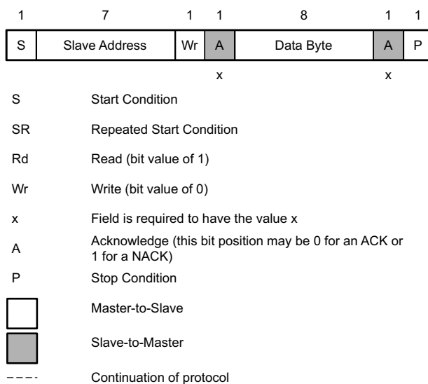
图 9-66. I²C Read/Write Protocol Key
