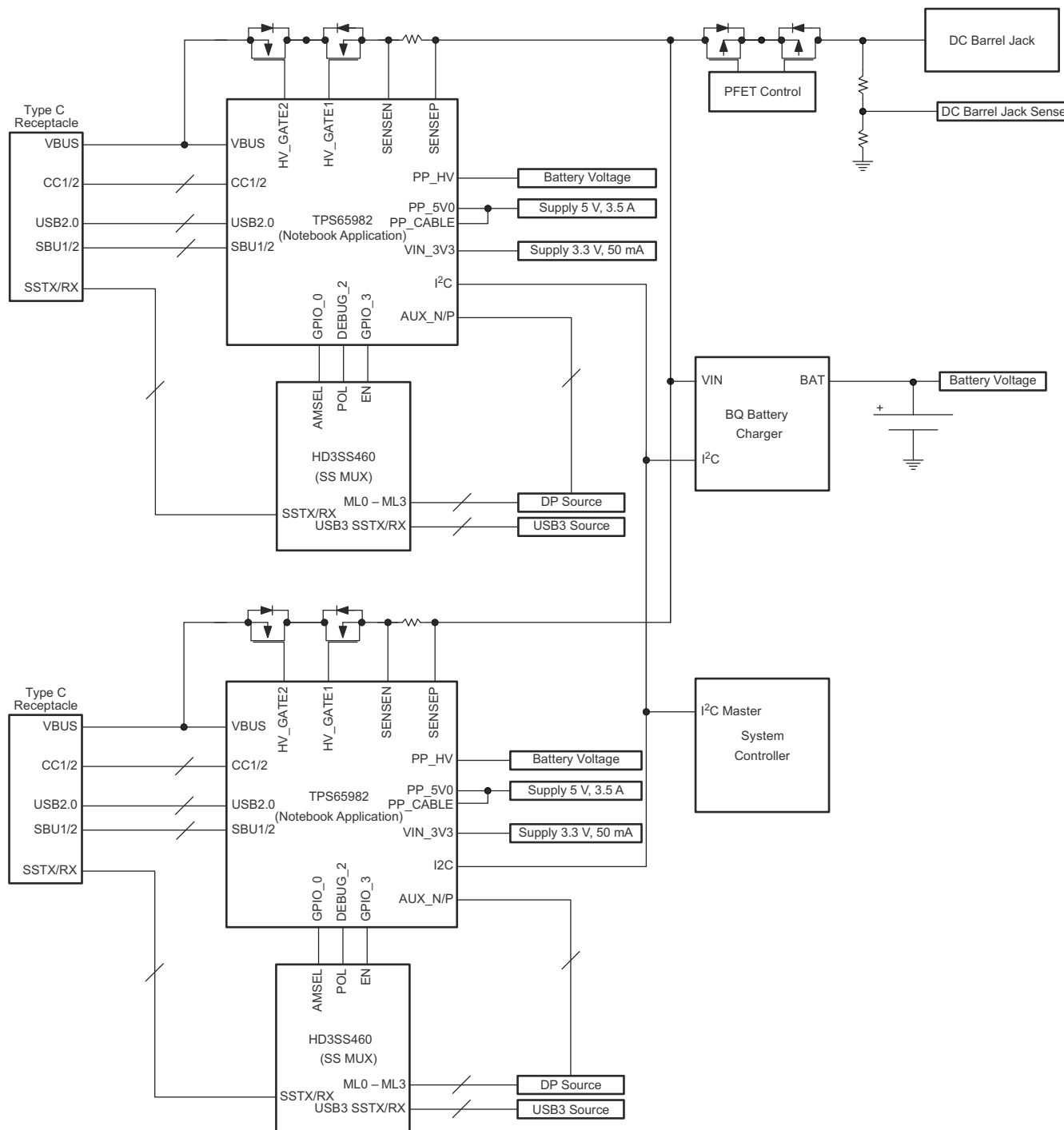
图 10-3. Dual-Port Notebook Application
