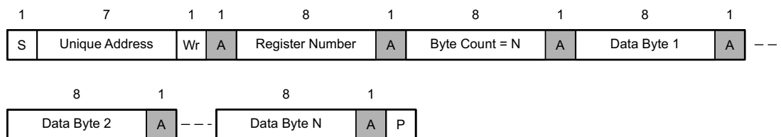
图 9-64. I²C Unique Address Write Register Protocol
