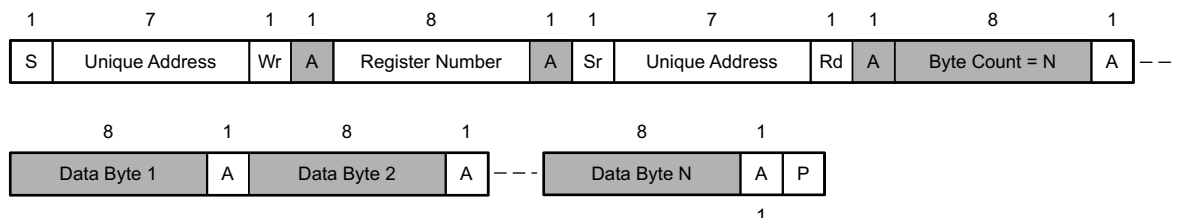
图 9-65. I²C Unique Address Read Register Protocol
