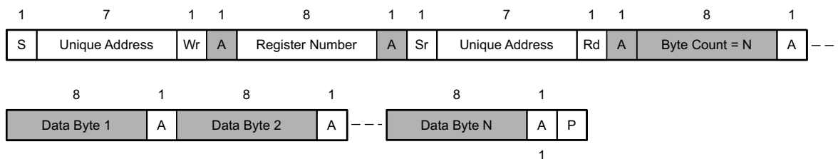
图 9-62. I 2 C Unique Address Read Register Protocol
