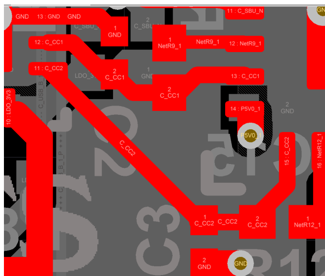
图 12-9. CC1 and CC2 Capacitor Routing
