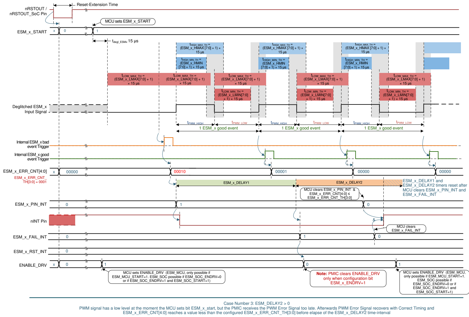
图 8-37. Example Waveform for ESM in PWM Mode - Case Number 3: ESM Starts with Low-Level at Deglitched Input Signal, but Receives Too Late a Correct PWM Signal Afterwards (The _x stand for _MCU or _SoC)
