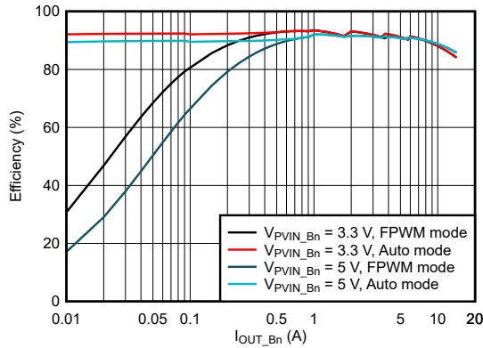
图 9-4. BUCK Efficiency at 3.3 V or 5 V Input Voltage
