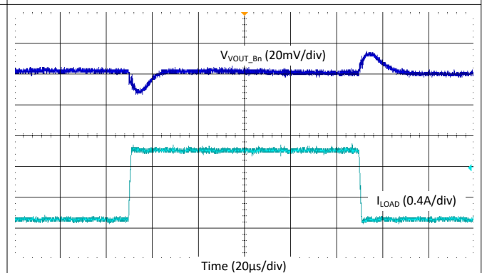
图 9-55. Buck Load Step Transient - Buck5, 4.4 MHz, Auto Mode
