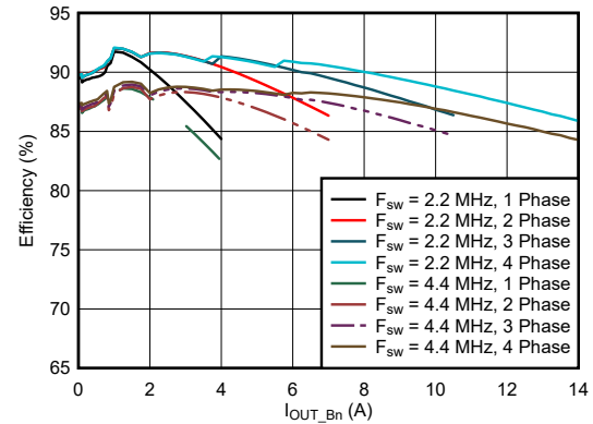
图 9-5. BUCK Efficiency with F_{sw} = 2.2\text{ MHz} or 4.4\text{ MHz}
