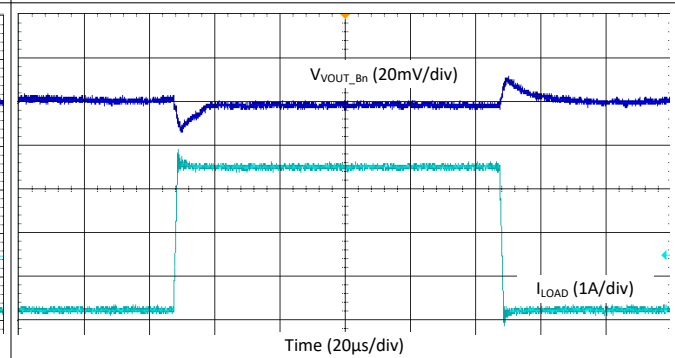
图 9-47. Buck Load Step Transient - 2-Phase, 4.4 MHz, Auto Mode
