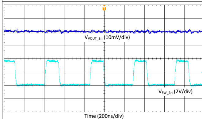
图 9-26. Buck Output Ripple - 2-Phase, Fsw = 2.2 MHz, Forced-PWM Mode
