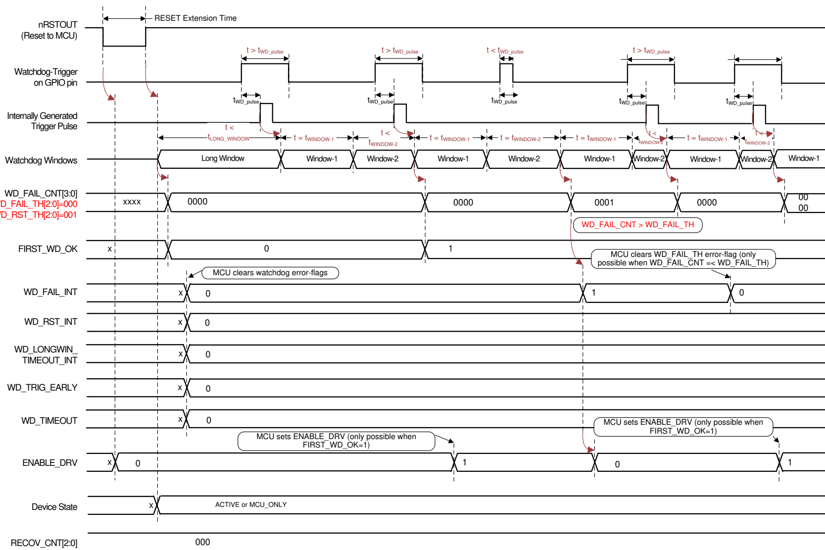
图 8-23. Watchdog in Trigger Mode – Good Events (Correct Watchdog-Triggers) After Start-up, Followed by a Bad-Event (No Watchdog-Trigger in Window-2) and After That Followed by a Good Event.
