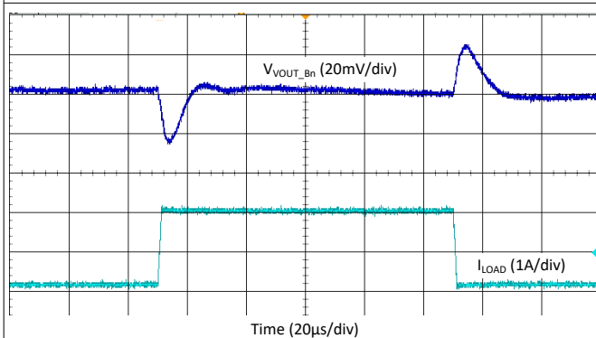
图 9-48. Buck Load Step Transient - 2-Phase, 2.2 MHz, Forced-PWM Mode
