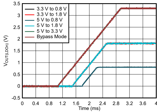
图 7-13. GPLDO Start-up with LDO_SLOW_RAMP = 1
