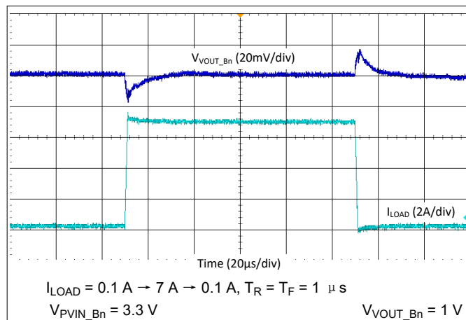
图 9-40. Buck Load Step Transient - 4-Phase, 2.2 MHz, Forced-PWM Mode
