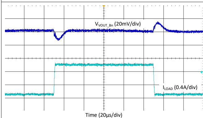
图 9-54. Buck Load Step Transient - Buck5, 2.2 MHz, Auto Mode
