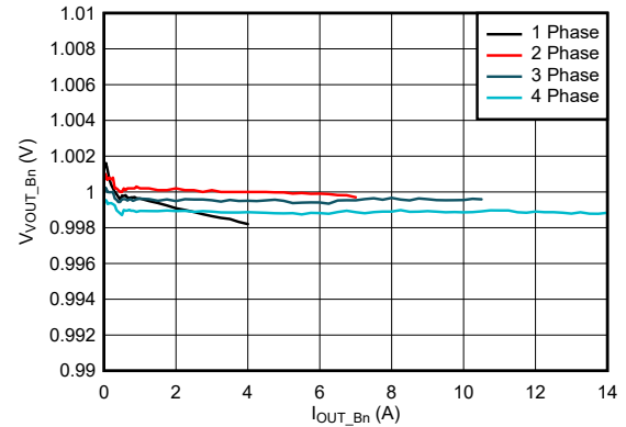
图 9-17. Buck Load Regulation with 5 V Input
