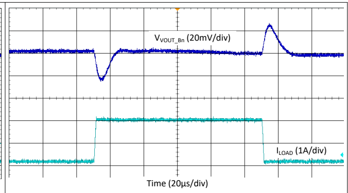
图 9-53. Buck Load Step Transient - Buck4, 4.4 MHz, Forced-PWM Mode
