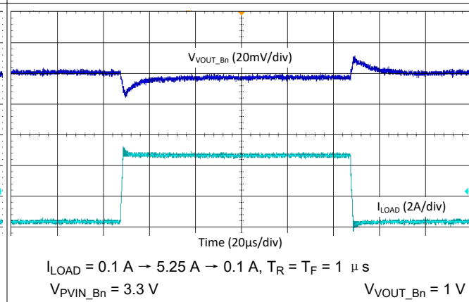
图 9-45. Buck Load Step Transient - 3-Phase, 4.4 MHz, Forced-PWM Mode
