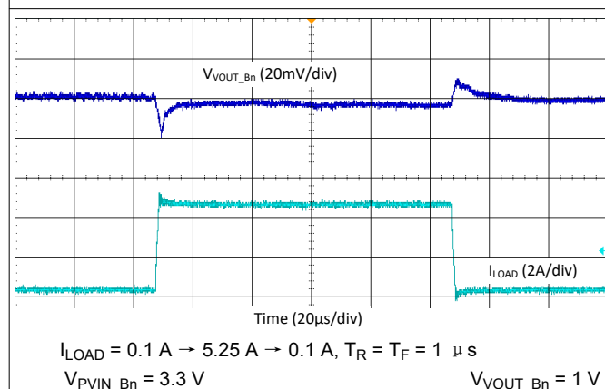
图 9-42. Buck Load Step Transient - 3-Phase, 2.2 MHz, Auto Mode
