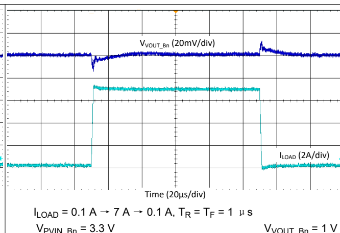
图 9-41. Buck Load Step Transient - 4-Phase, 4.4 MHz, Forced-PWM Mode
