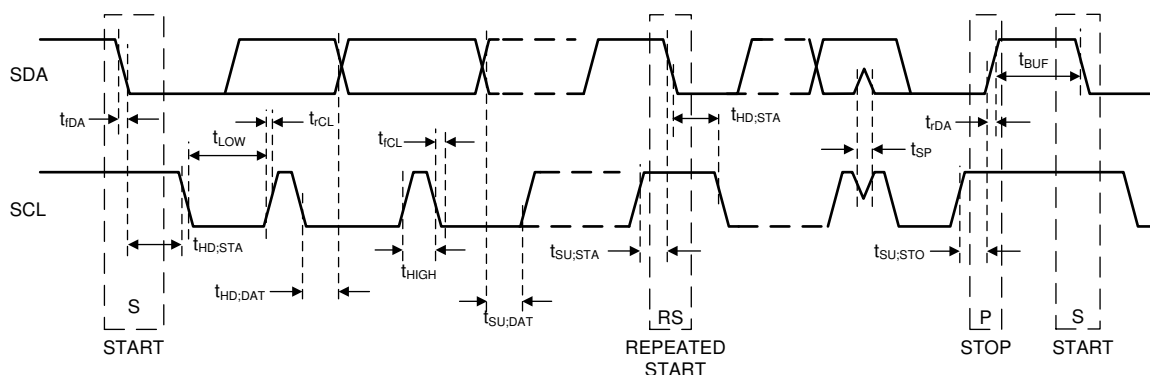
图 8-55. I²C-Compatible Timing
