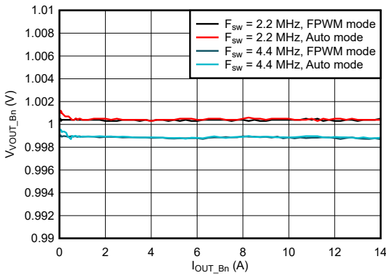
图 9-16. Buck Load Regulation with 3.3 V Input
