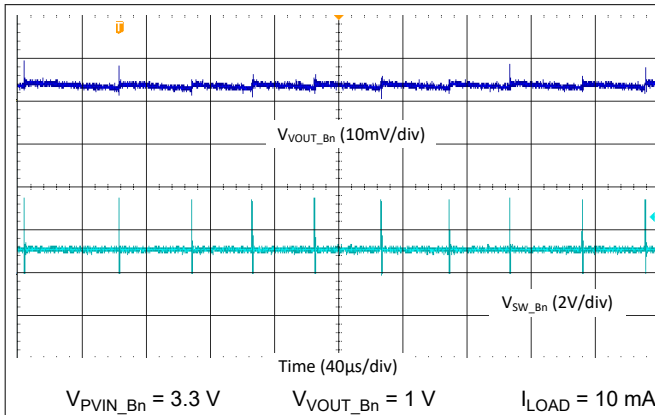
图 9-28. Buck Output Ripple - 3-Phase, Auto Mode
