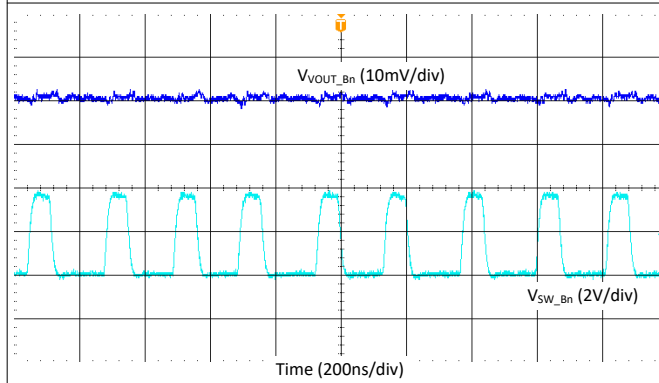
图 9-24. Buck Output Ripple - Single Phase, Fsw = 4.4 MHz, Forced-PWM Mode
