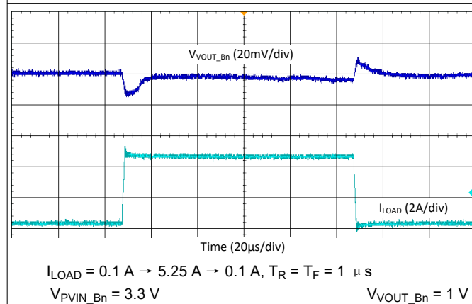
图 9-44. Buck Load Step Transient - 3-Phase, 2.2 MHz, Forced-PWM Mode
