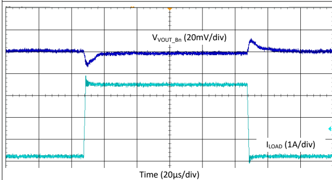
图 9-46. Buck Load Step Transient - 2-Phase, 2.2 MHz, Auto Mode
