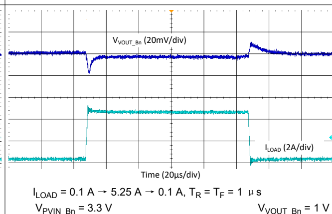
图 9-43. Buck Load Step Transient - 3-Phase, 4.4 MHz, Auto Mode
