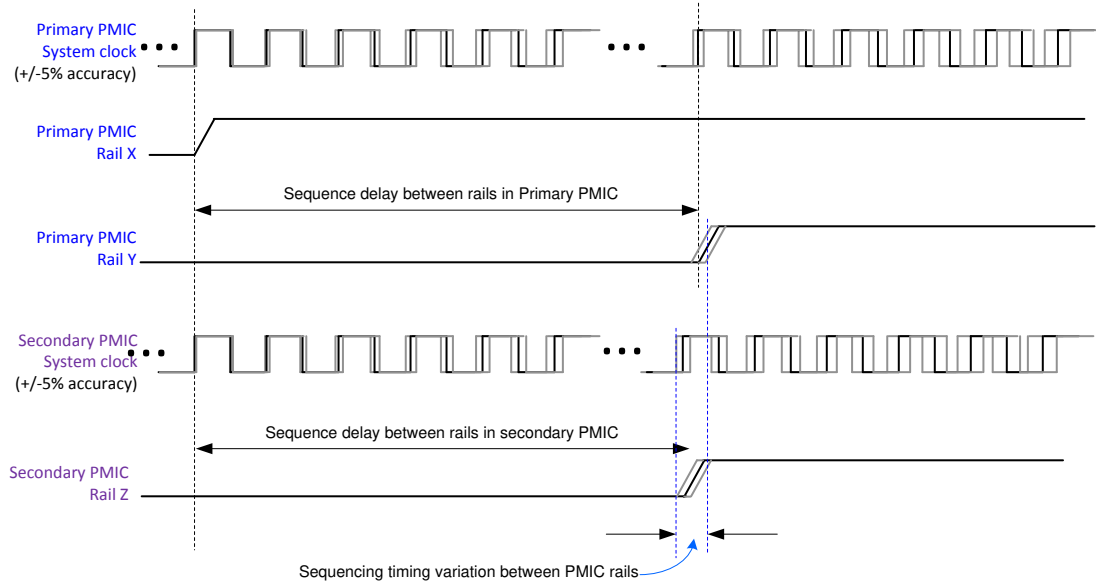
图 8-48. Multi-PMIC Rail Sequencing Timing Variation
