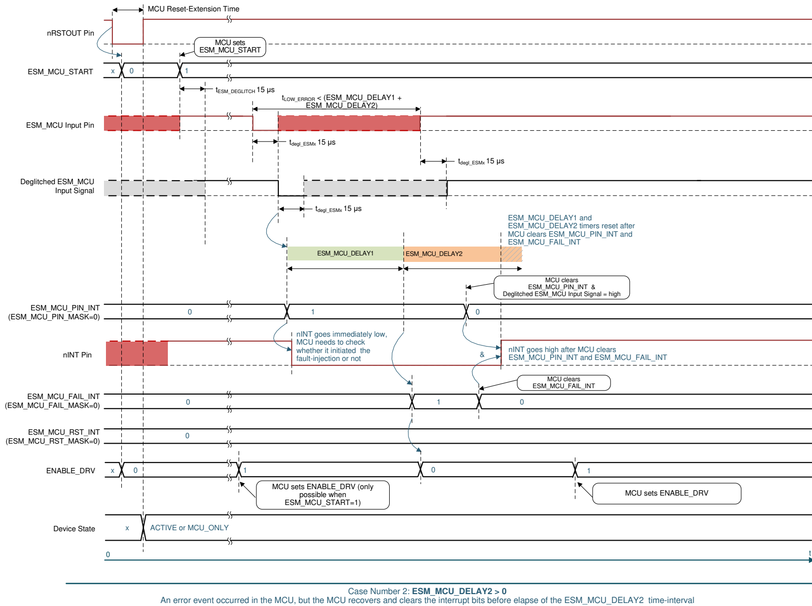
图 8-30. Example Waveform for ESM in Level Mode - Case Number 2: Delay-2 Not Set To 0 and ESM_MCU_ENDRV=1, ESM_MCU Signal Recovers Elapse of Delay-2 Time-Interval
