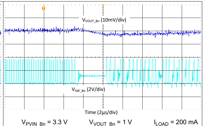
图 9-35. Buck Transient from PWM mode to PFM mode, 4.4 MHz, Single Phase
