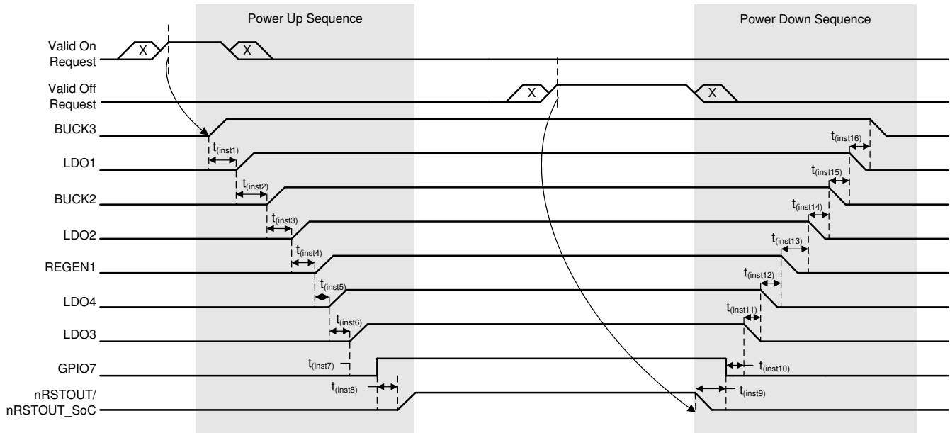
图 8-45. Power Sequence Example
