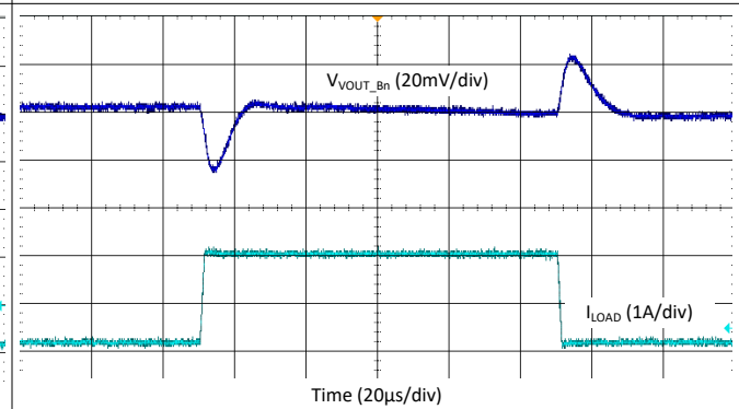
图 9-49. Buck Load Step Transient - 2-Phase, 4.4 MHz, Forced-PWM Mode
