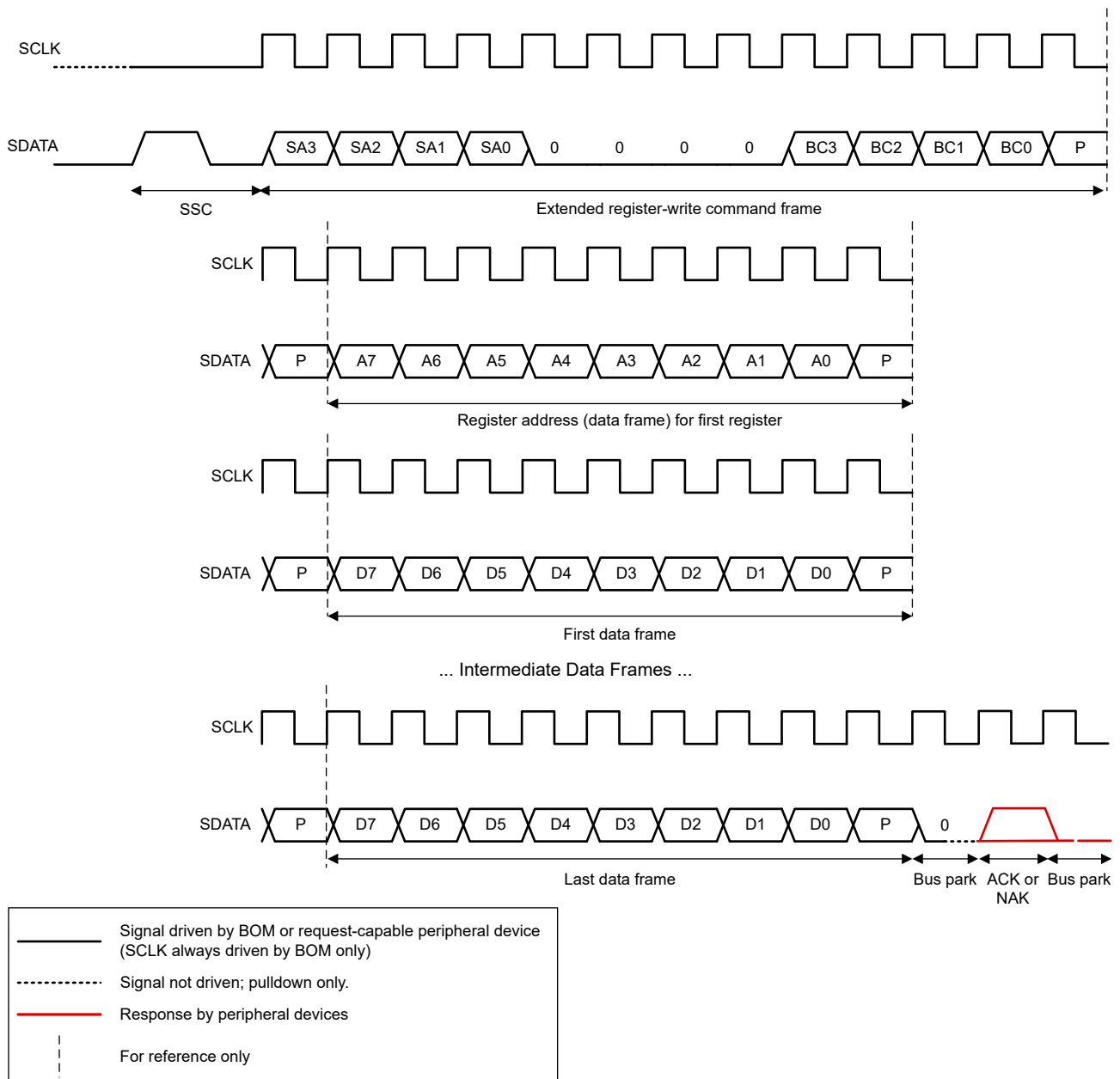
图 8-49. SPMI Extended Register Write Command
