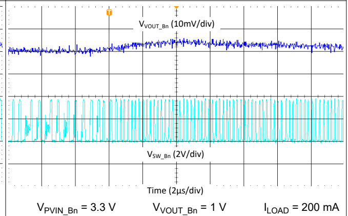
图 9-37. Buck Transient from PFM mode to PWM mode, 4.4 MHz, Single Phase
